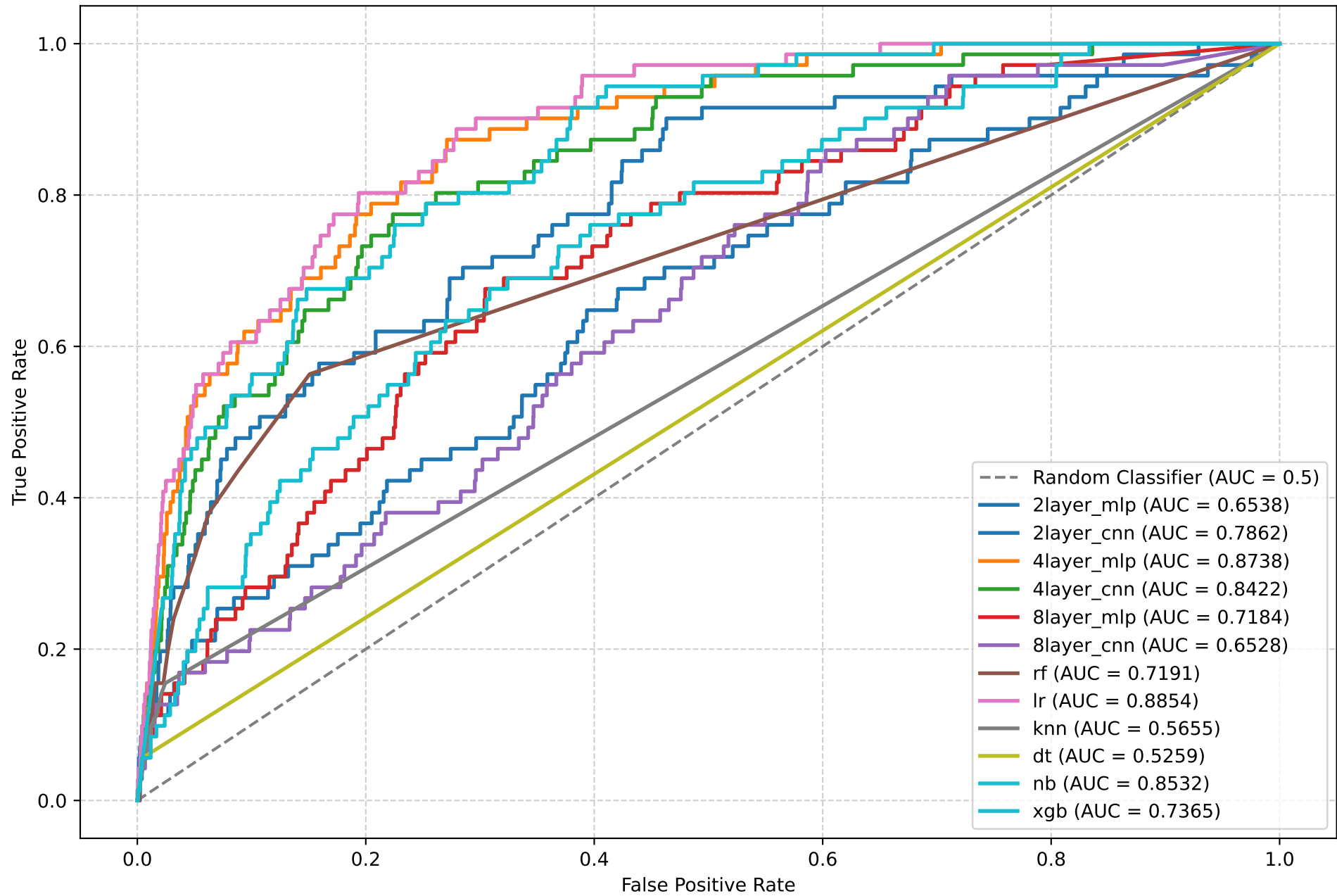
ROC Curve - FAILWEAN
