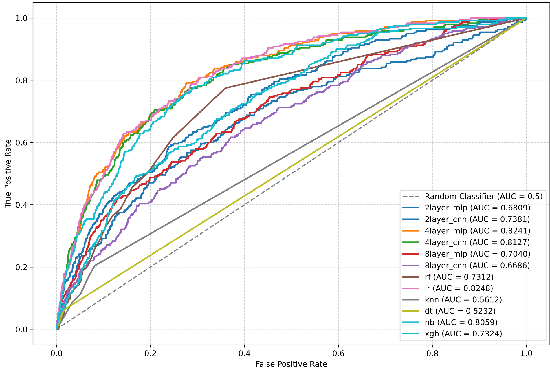
ROC Curve - OUPNEUMO
