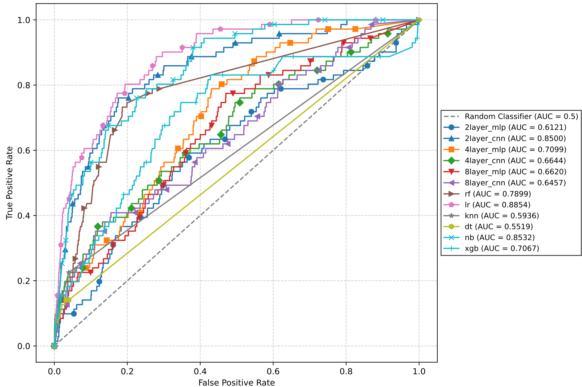
ROC Curve - FAILWEAN (Best Models)
