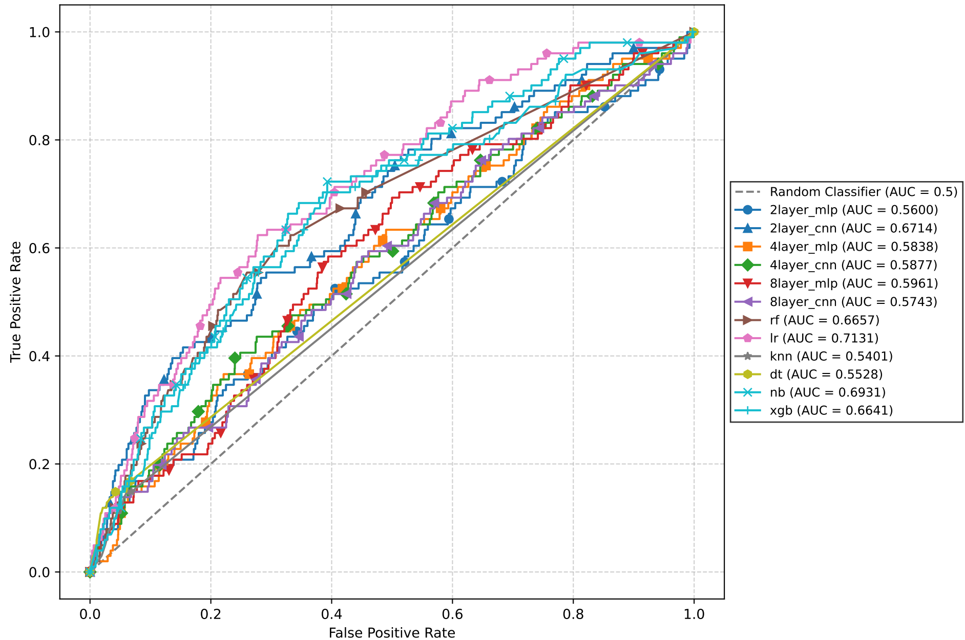
ROC Curve - PULEMBOL (Best Models)
