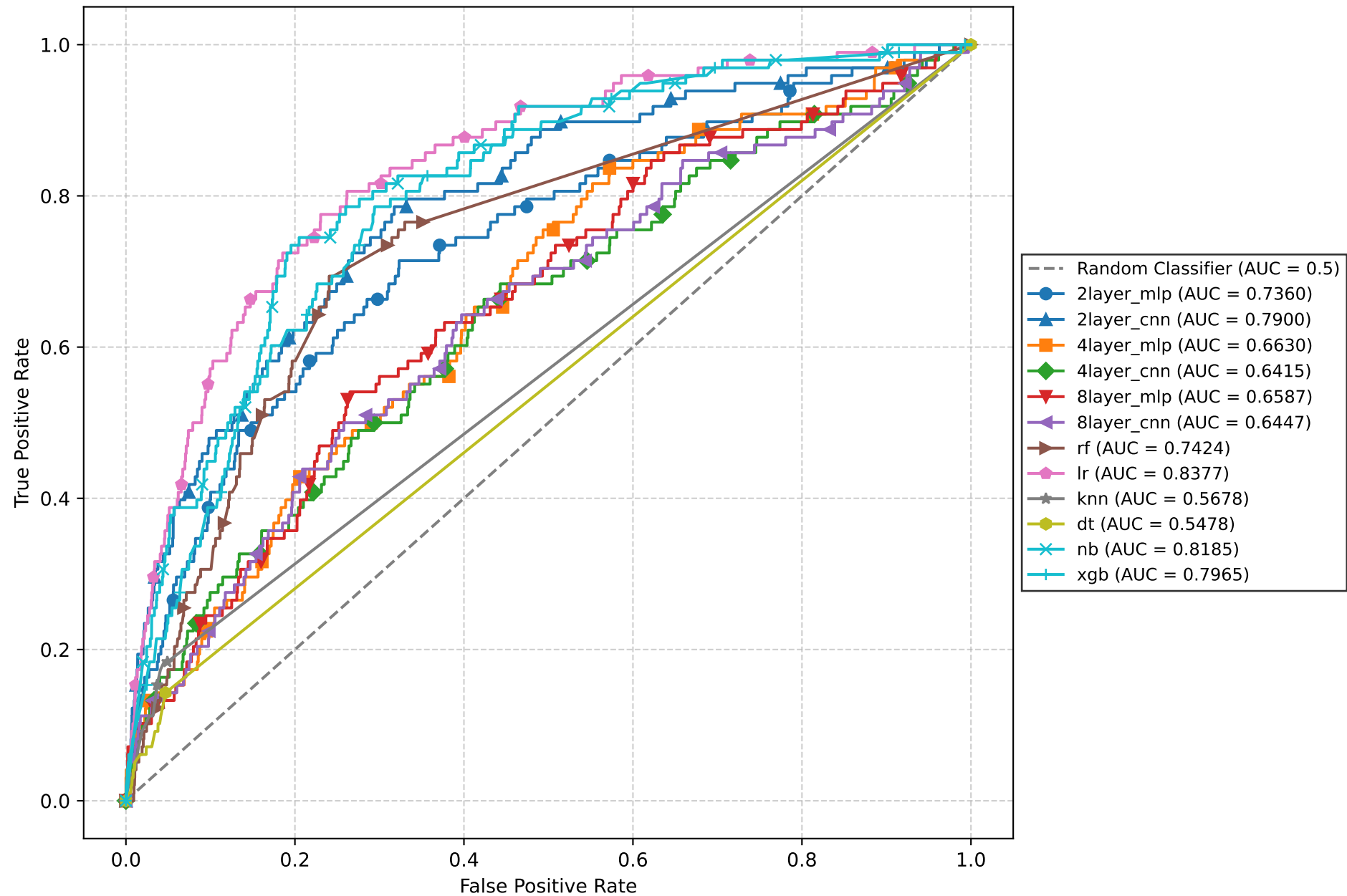
ROC Curve - REINTUB (Best Models)
