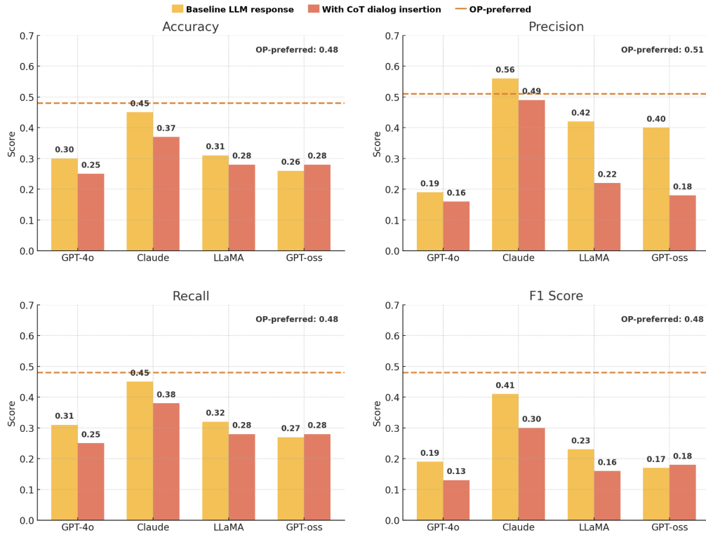
Figure 5.1: r/aitah —Overall performance scores (Accuracy, Precision, Recall, and F1 Score) for OP-preferred responses and model outputs (GPT-4o, Claude, LLaMA, GPT-oss), comparing model baseline response with CoT dialog insertion. Values represent aggregate scores across the four classes, not per-class results.
