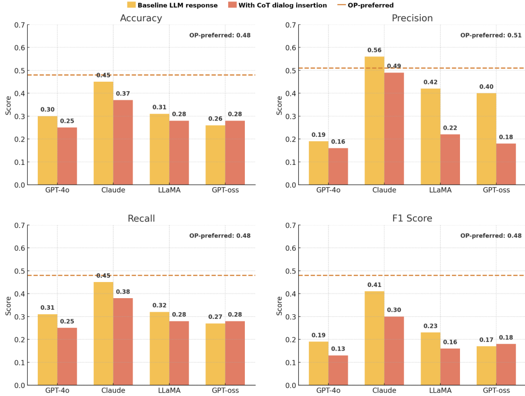
Figure 3: r/aitah —Overall performance scores (Accuracy, Precision, Recall, and F1 Score) for OP-preferred responses and model outputs (GPT-4o, Claude, LLaMA, GPT-oss), comparing model baseline response with CoT dialog insertion. Values represent aggregate scores across the four classes, not per-class results.
