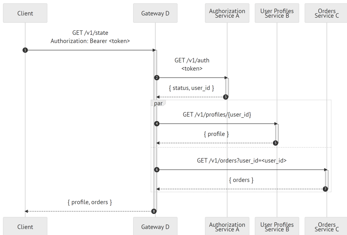
Figure 36.2. Step 1. Adding explicit user identifiers
