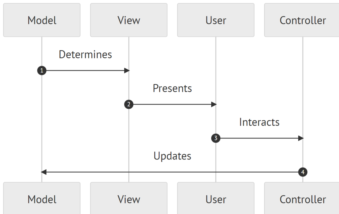
Figure 44.1. MVC entities interaction chart
