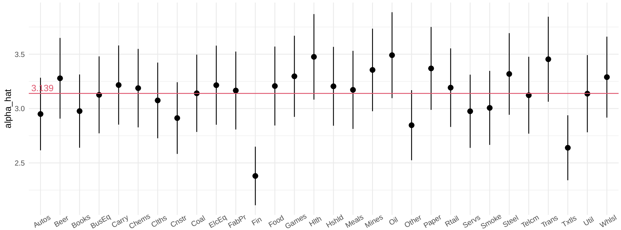
Confidence Intervals for alpha with k=300
