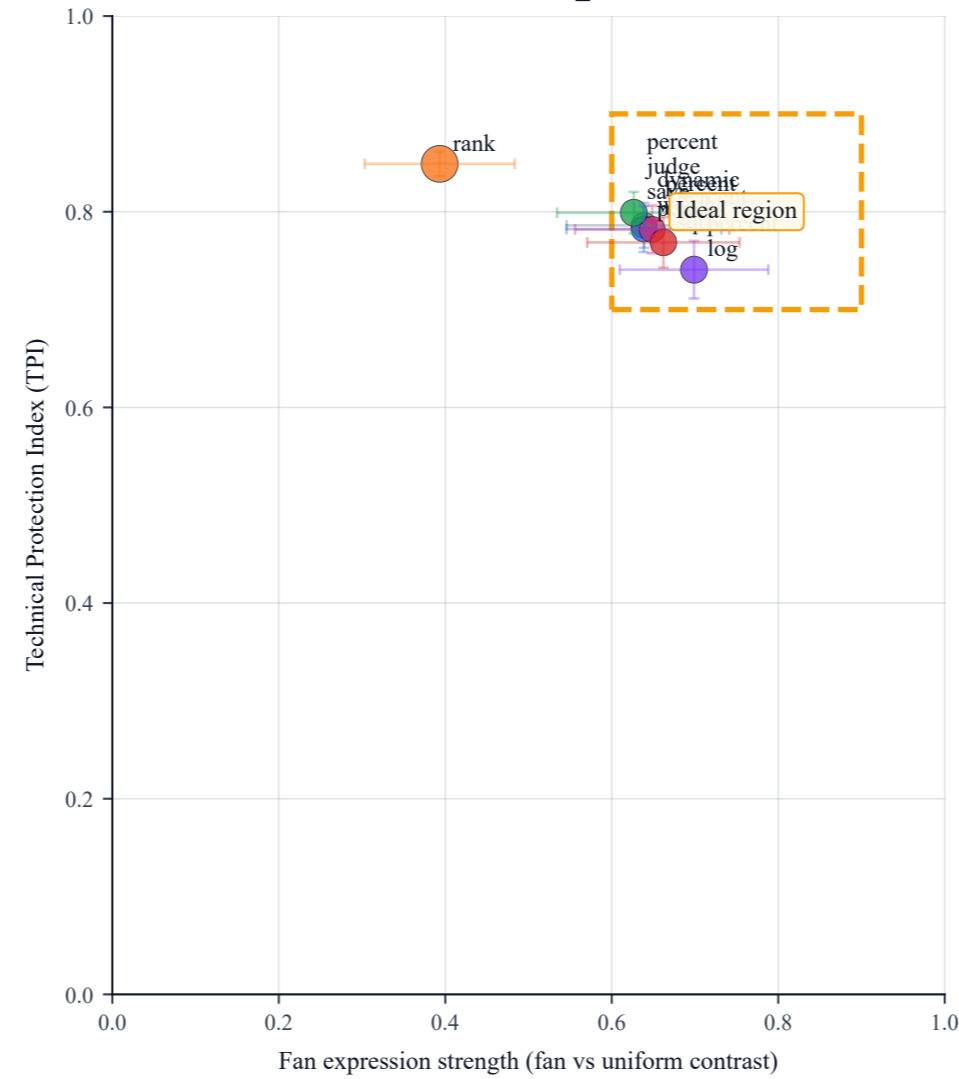
Stress test: outlier_mult=5.0
