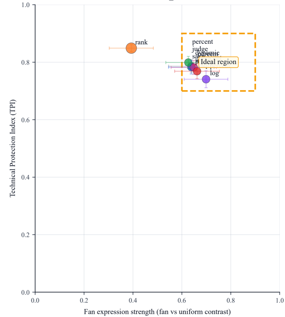
Stress test: outlier_mult=10.0
