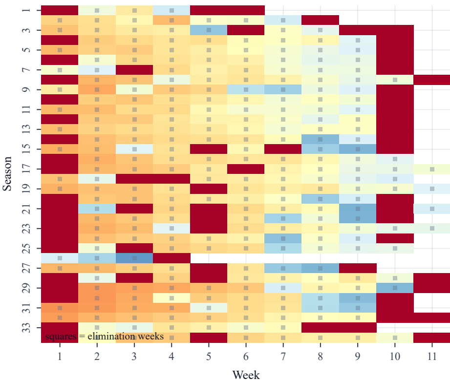
ESS Ratio (Lower = Higher Uncertainty)
