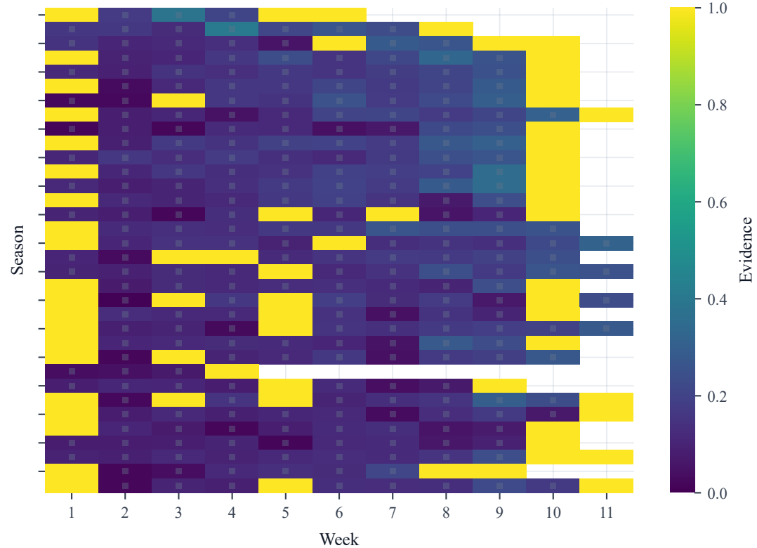
Evidence (Brighter = Stronger Constraints)
