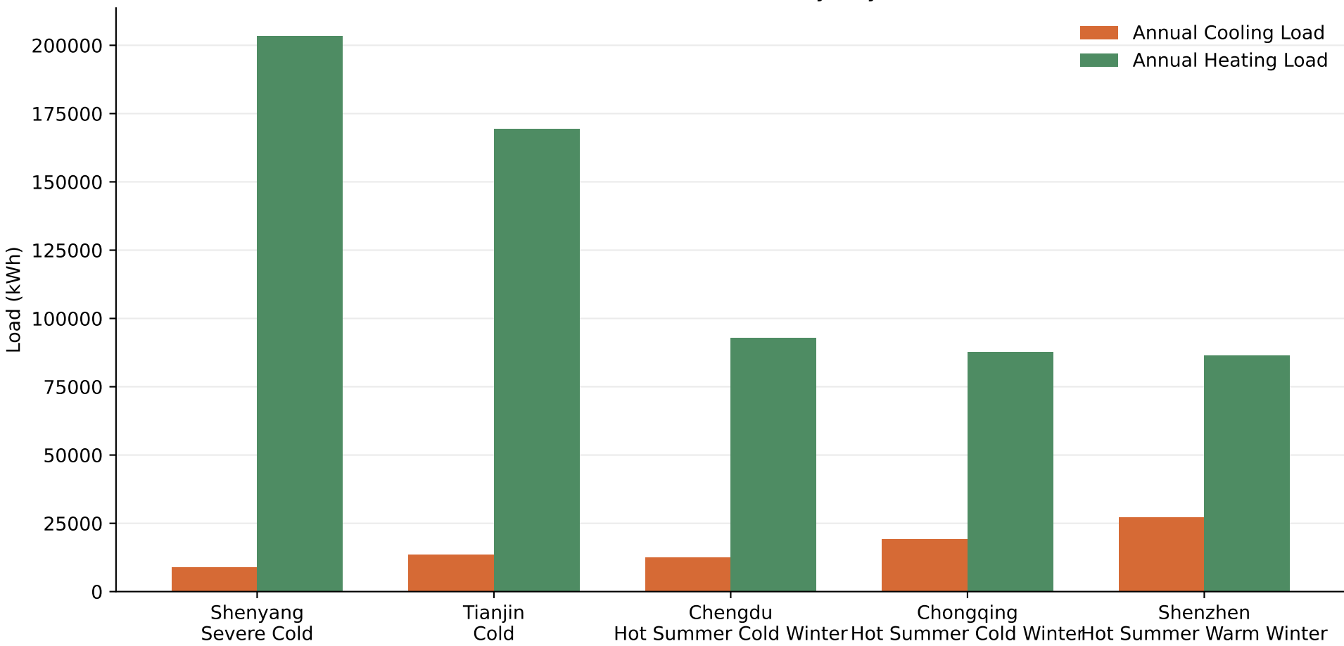
Annual Ideal Loads by City
