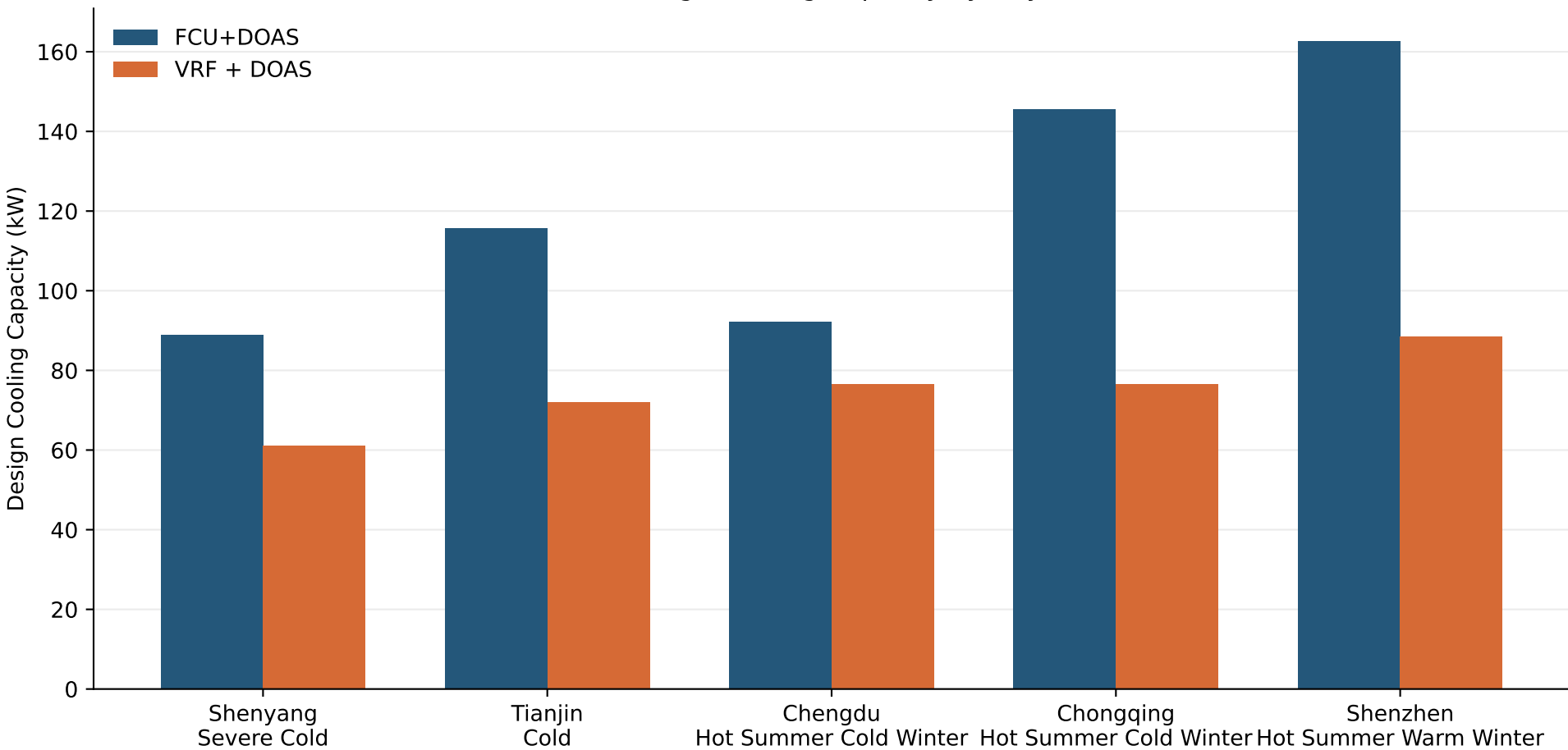
Design Cooling Capacity by City
