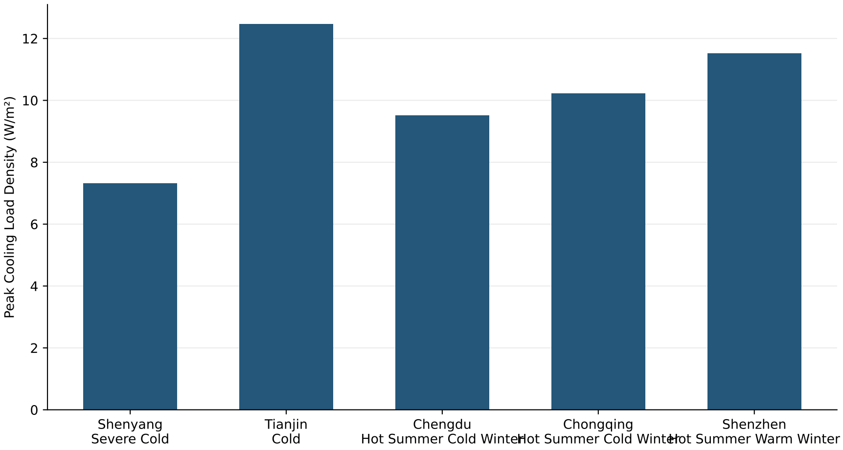
Peak Cooling Load Density by City
