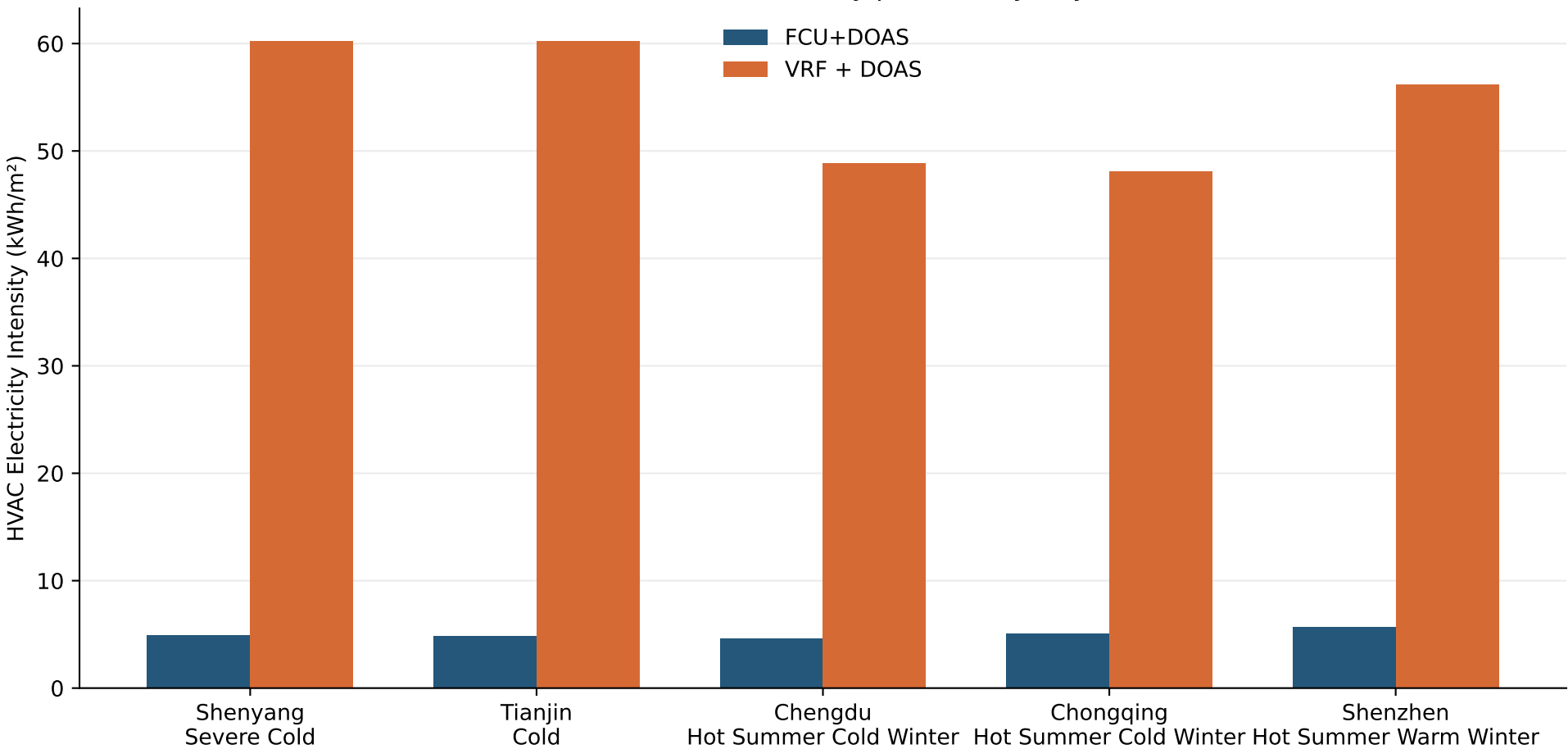
Annual HVAC Electricity per Area by City
