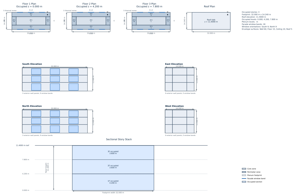
IDF-Derived Medium Office Building Structure Plan, roof, facade, and section views reconstructed from EnergyPlus model geometry
