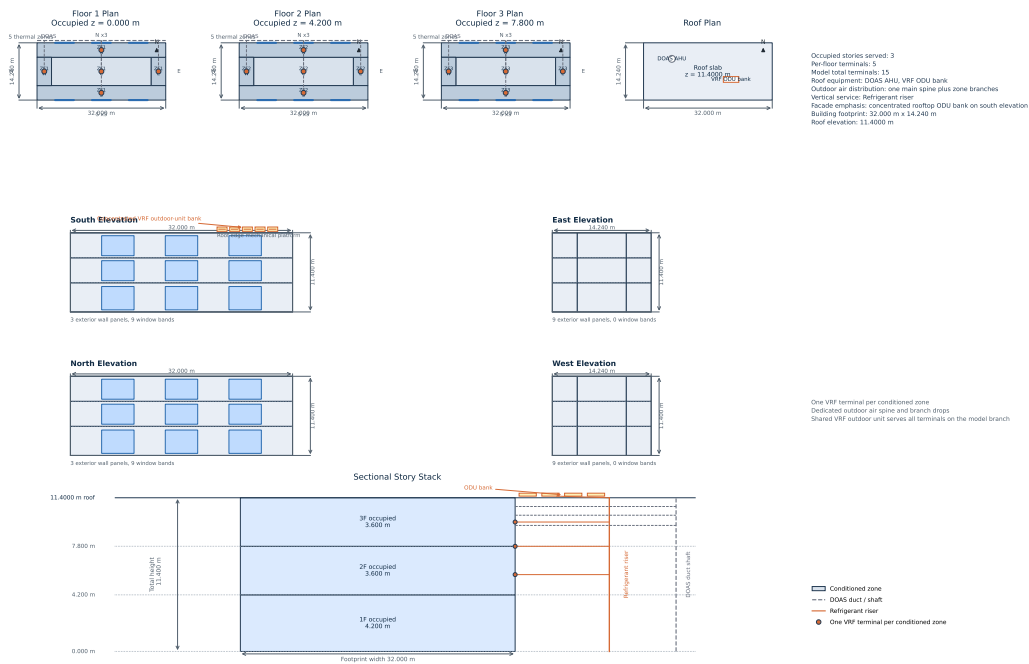
VRF + DOAS Service Overlay
