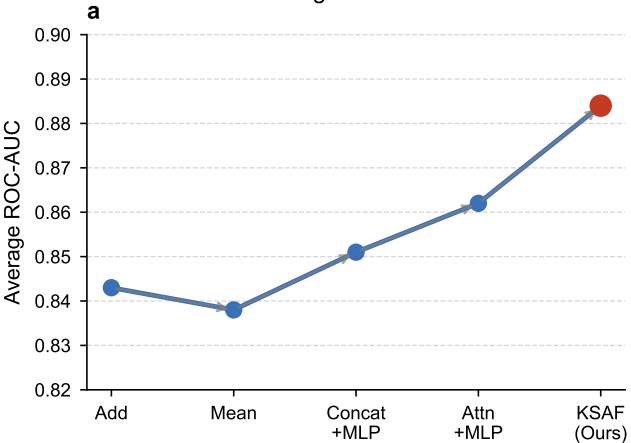
Progressive Performance Evolution of Local-Global Fusion Architectures
