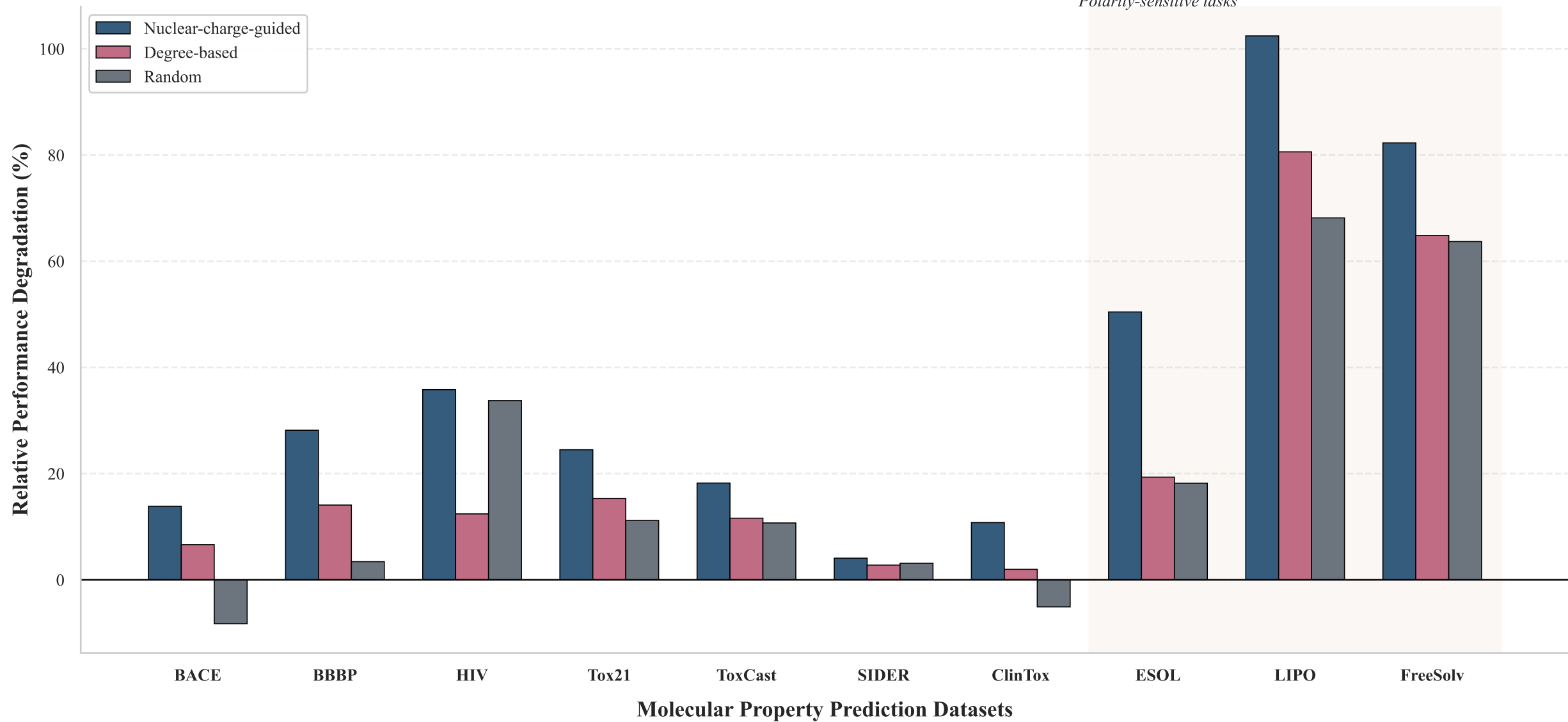
Sensitivity to Atomic-Semantic Perturbation under Different Node Ordering Strategies
