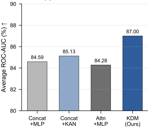
(a) Classification benchmarks
