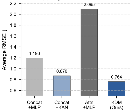
(b) Regression benchmarks
