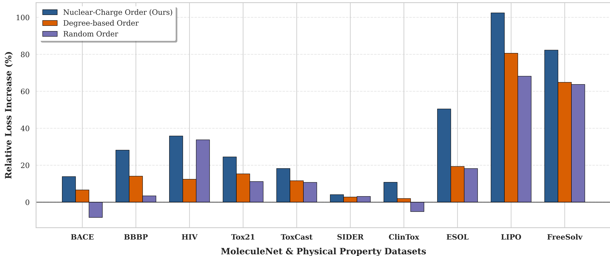
Permutation Feature Importance (PFI) of Atomic Number Z under Different Node Orderings
