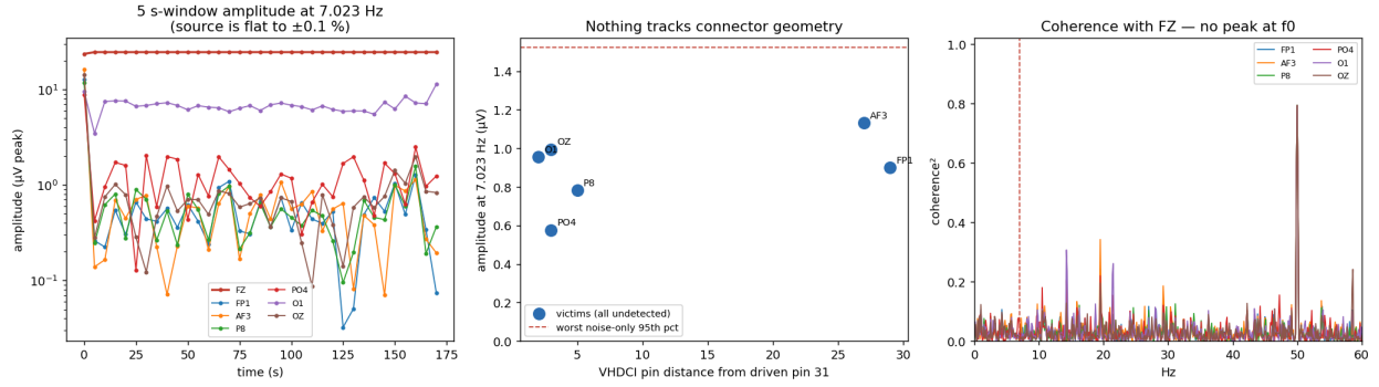
Figure 4: Left: 5s-window amplitude at f_0 ; the source is flat, the floating channels wander around 1 \mu\text{V} with no relationship to it. Centre: amplitude against VHDCI pin distance from the driven pin. Right: magnitude-squared coherence with the driven channel — no peak at f_0 .
