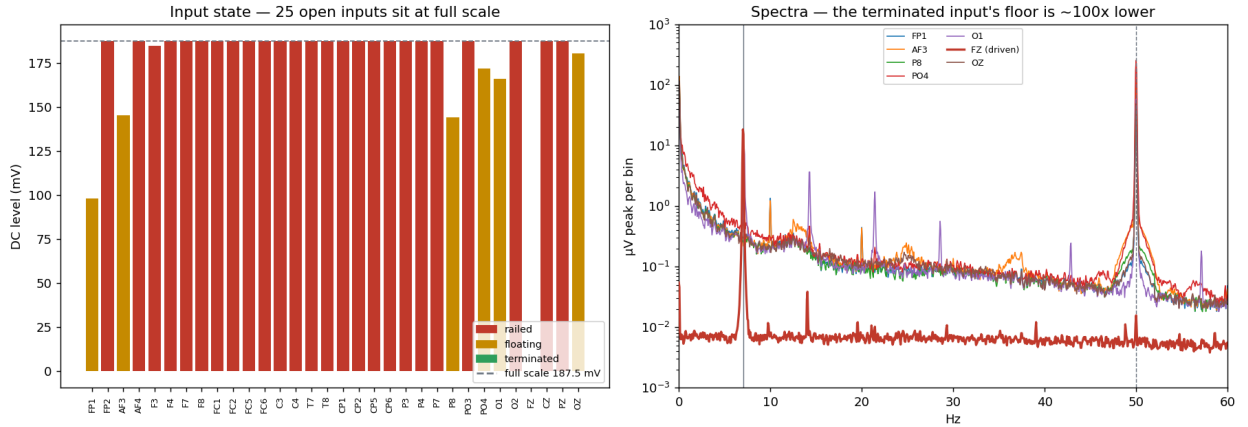
Figure 1: Left: DC level per input. Twenty-five inputs sit exactly at full scale. Right: amplitude spectra of the seven channels that are not saturated. The terminated channel (red) has a noise floor roughly two decades below the floating ones and essentially no 50 Hz; the floating channels carry 3.5 to 26.5\,\mu\text{V} of mains and a large low-frequency drift skirt.
