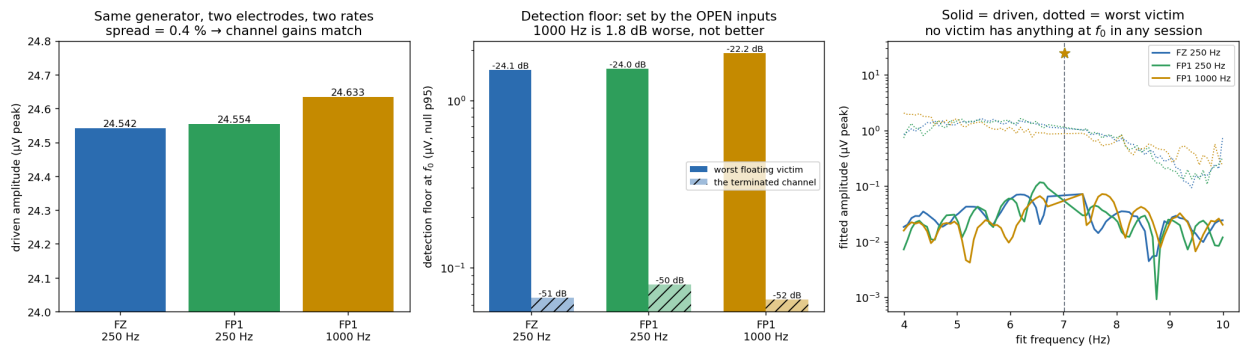
Figure 6: Left: driven amplitude across the three sessions — 0.37 % total spread. Centre: the detection floor, split into the terminated channel (hatched) and the worst floating one. The gap between them, roughly 27 dB, is the entire cost of leaving inputs open. Right: the frequency sweep for all three sessions overlaid; solid is the driven channel, dotted is that session’s worst victim. Every dotted curve passes smoothly through f_0 .
