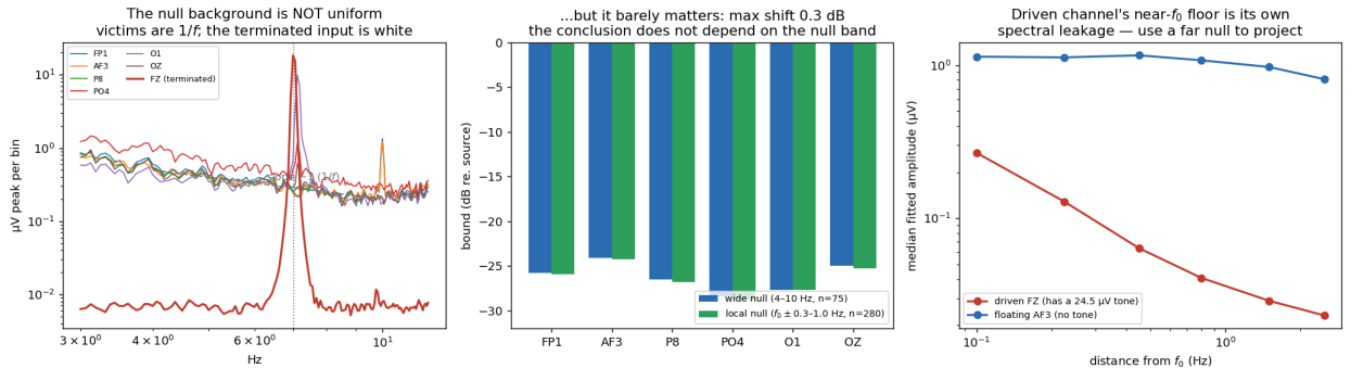
Figure 5: Left: the background over the null band. Every floating channel follows 1/f ; the one terminated channel is white there (slope +0.21 ), which is what a properly biased input should look like. Centre: the bound computed from the wide null against a local null hugging f_0 . Right: the driven channel’s fitted amplitude against distance from f_0 — a monotonic decay that is leakage from its own tone, absent on a channel that carries no tone.
