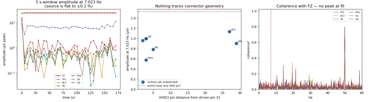
Figure 4: Left: 5s-window amplitude at f_0 ; the source is flat, the floating channels wander around 1\mu\text{V} with no relationship to it. Centre: amplitude against VHDCI pin distance from the driven pin. Right: magnitude-squared coherence with the driven channel — no peak at f_0 .
