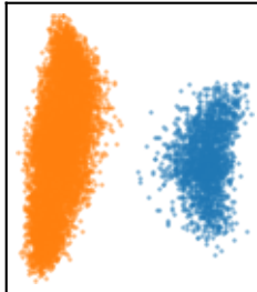
coco-t2i
