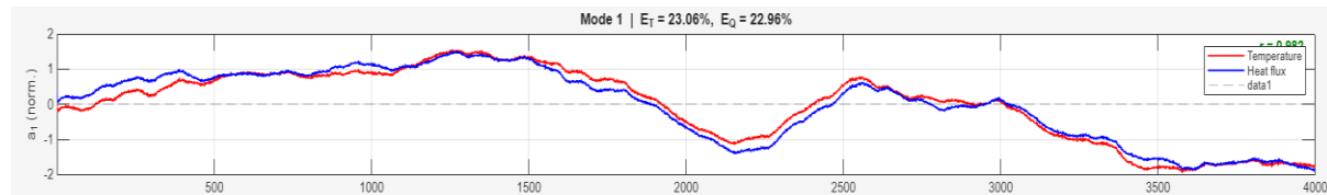
Figure 8 - Mode 1 heat flux and temperature coefficients overlayed
