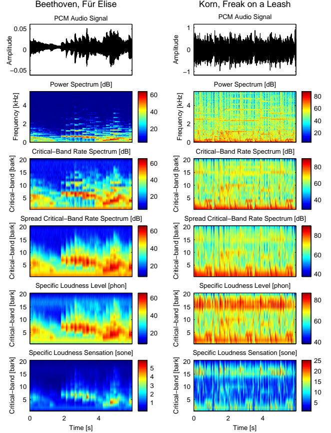
Figure 2: Steps S1-S6: from the 11kHz PCM audio signal to specific loudness per critical-band
