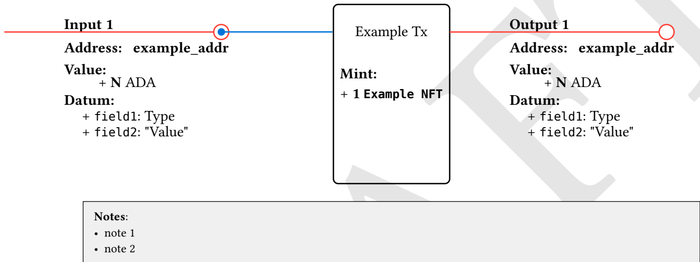
Figure 1: Example transaction
