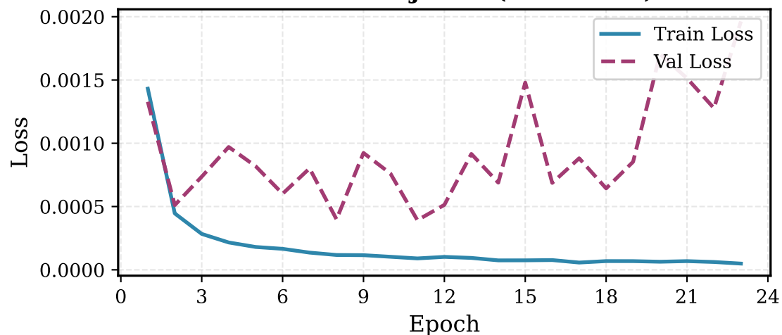
Best #1: Subject 9 (F1=98.3%)
