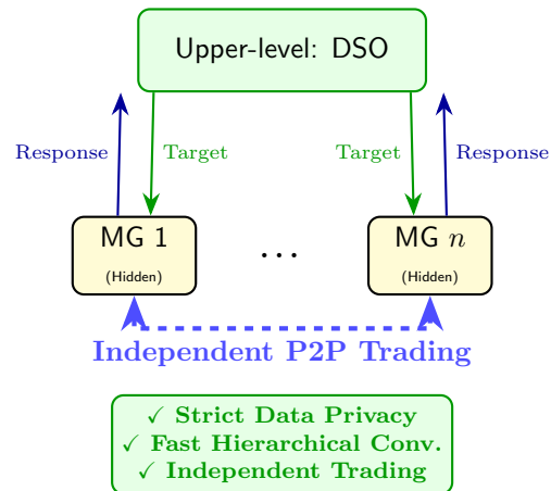
(c) Proposed Hierarchical ATC
