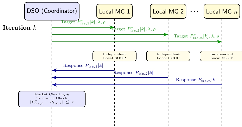
(d) ATC Iterative Sequence Flow: Secure &amp; Independent P2P Coordination
