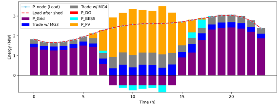
(b) Active Power MG2
