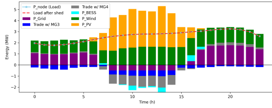
(a) Active Power MG1
