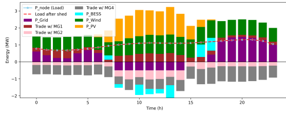
(c) Active Power MG3
