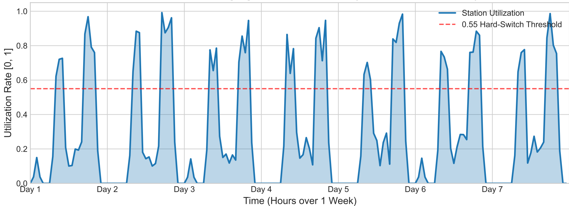
Real-World EV Charging Station Utilization (Bimodal Peak Pattern)
