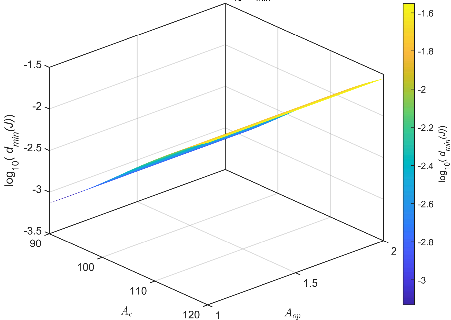
3D surface of \log_{10}(d_{min}(J))
