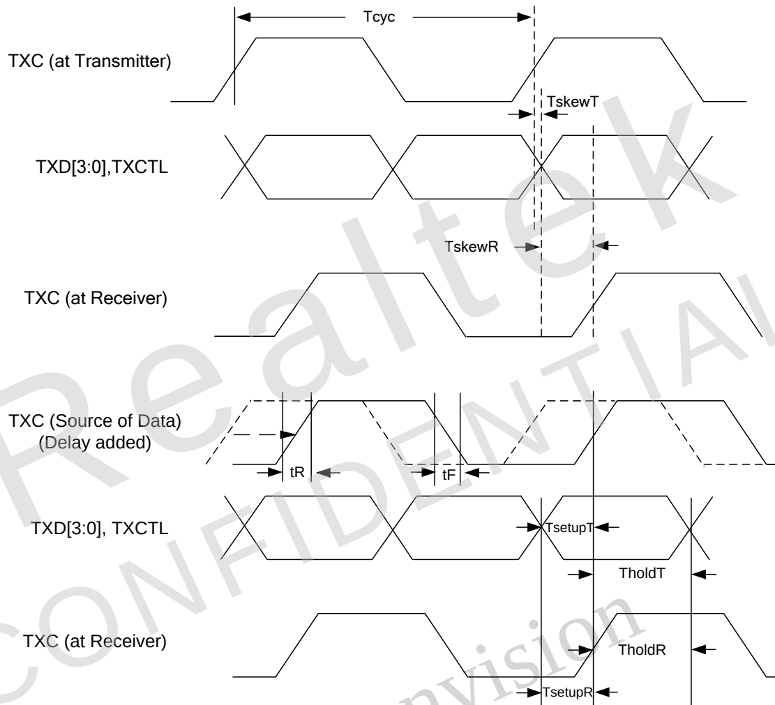
Figure 14. RGMII Timing Modes (For TXC)
