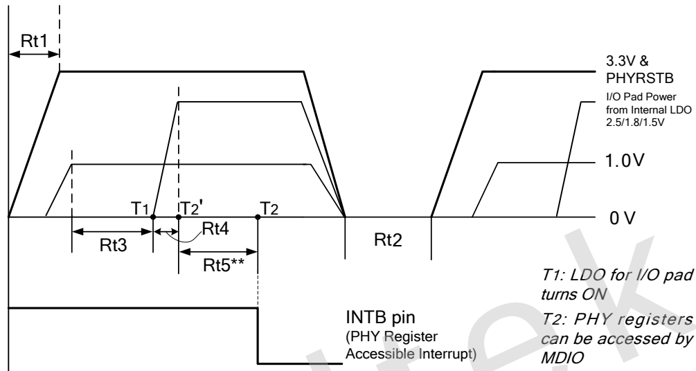
Figure 10. Power Sequence (I/O Pad Power Sourced from Internal LDO)
