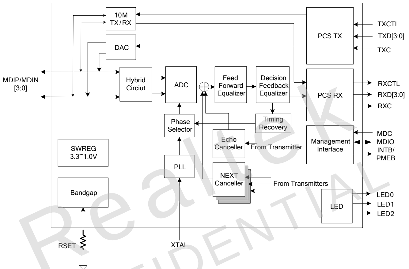
Figure 3. Block Diagram
