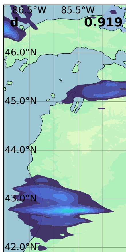
LESNet-A
