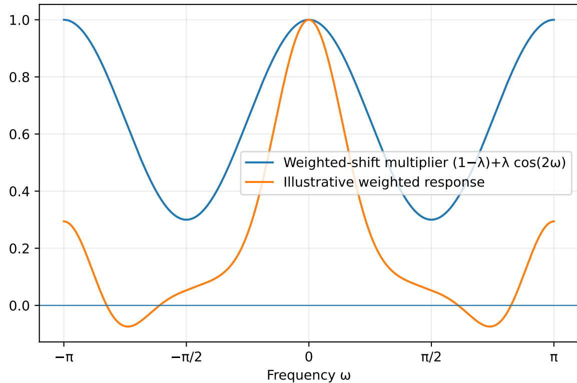
p=2 weighted-shift spectral modulation
