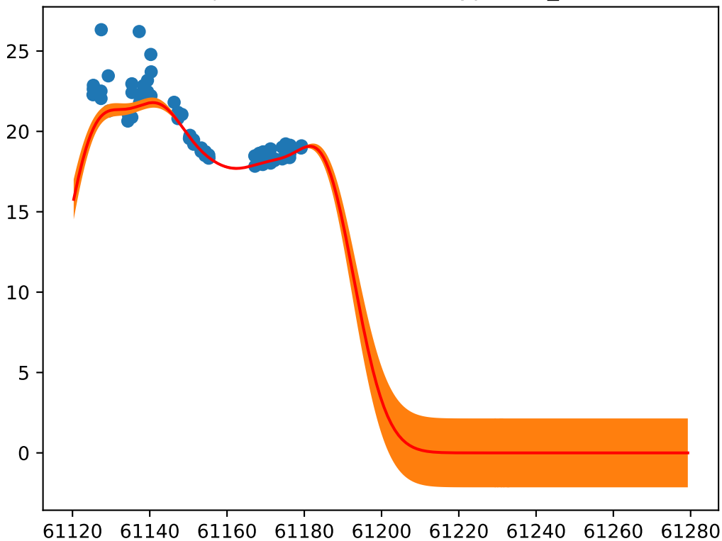
Object: ZTF26aatmcni; Type: SN_Ia
