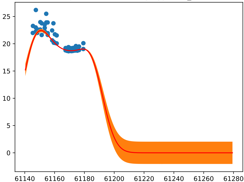
Object: ZTF26aauxkmg; Type: SN_Ia
