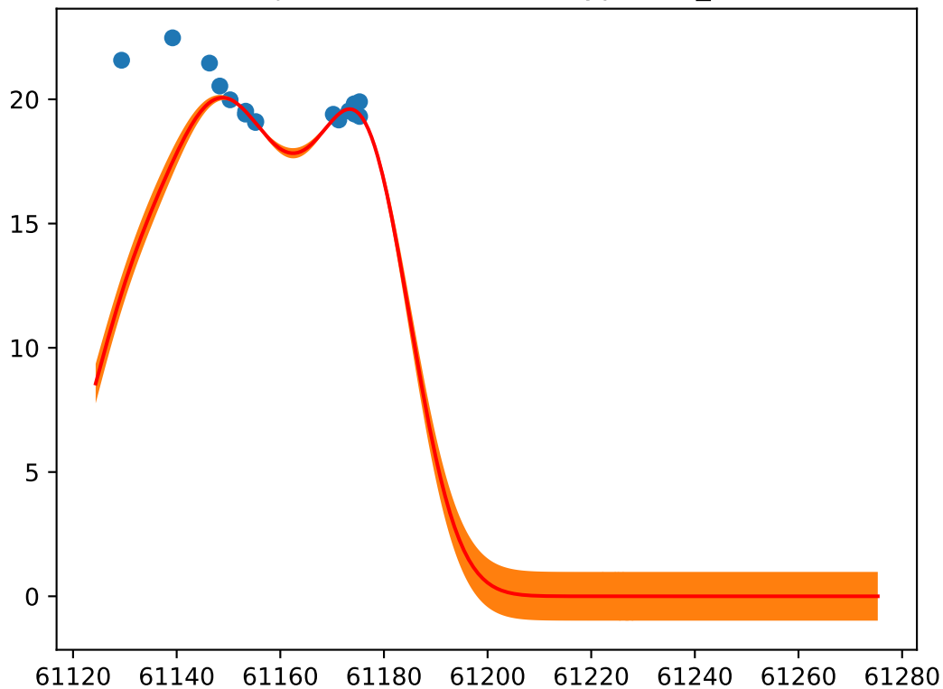
Object: ZTF26aatktdb; Type: SN_Ia
