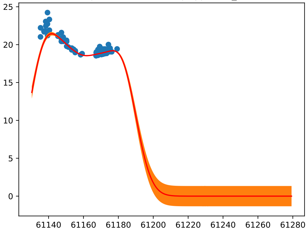
Object: ZTF26aatvsoq; Type: SN_Ia
