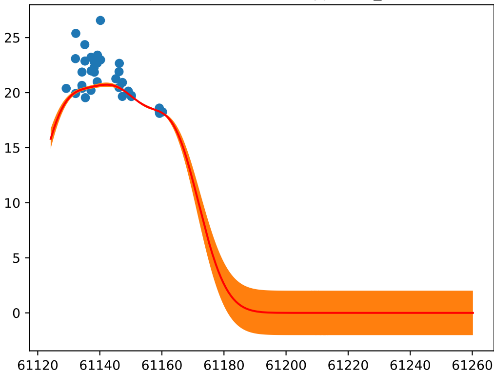
Object: ZTF26aatifnw; Type: SN_Ia
