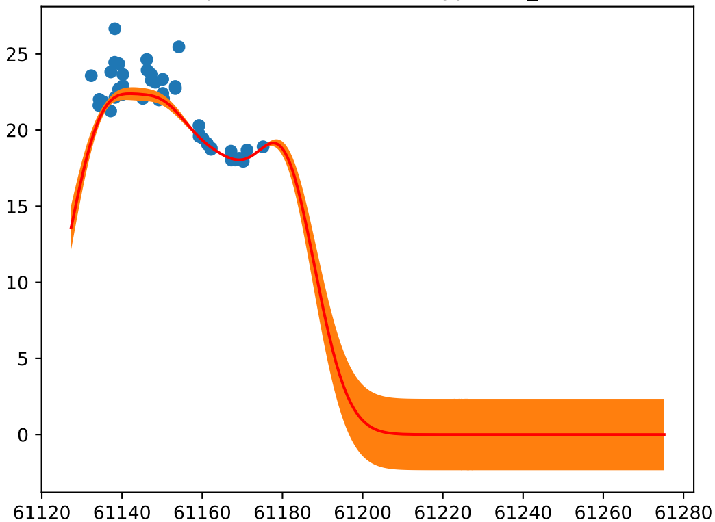
Object: ZTF26aaulhso; Type: SN_Ia
