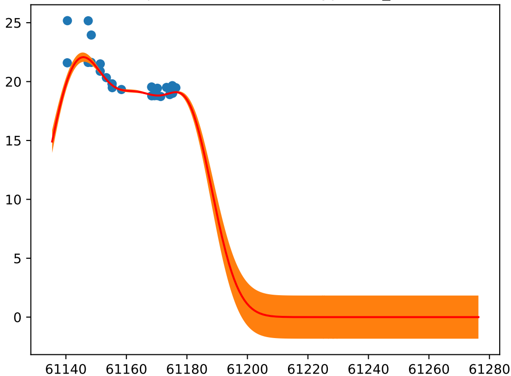
Object: ZTF26aatweku; Type: SN_Ia
