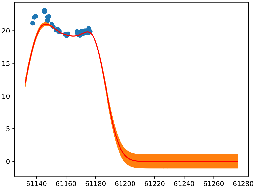
Object: ZTF26aadaac; Type: SN_Ia
