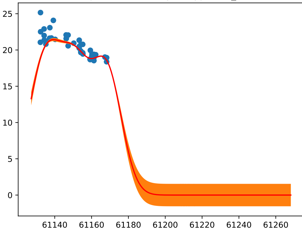
Object: ZTF25aateyv; Type: SN_Ia
