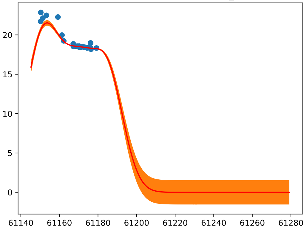
Object: ZTF26aaurvzt; Type: SN_Ia
