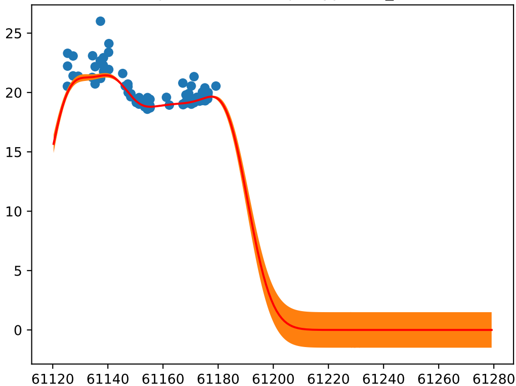
Object: ZTF19aaloljd; Type: SN_Ia
