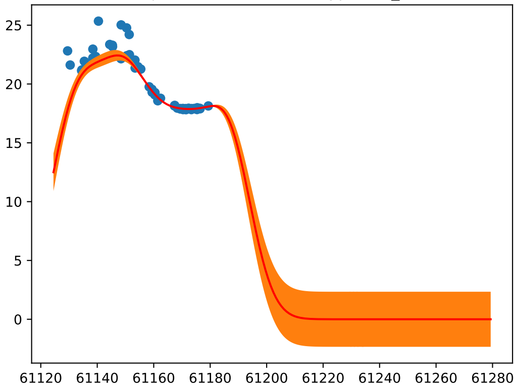
Object: ZTF26aaumtdl; Type: SN_Ia
