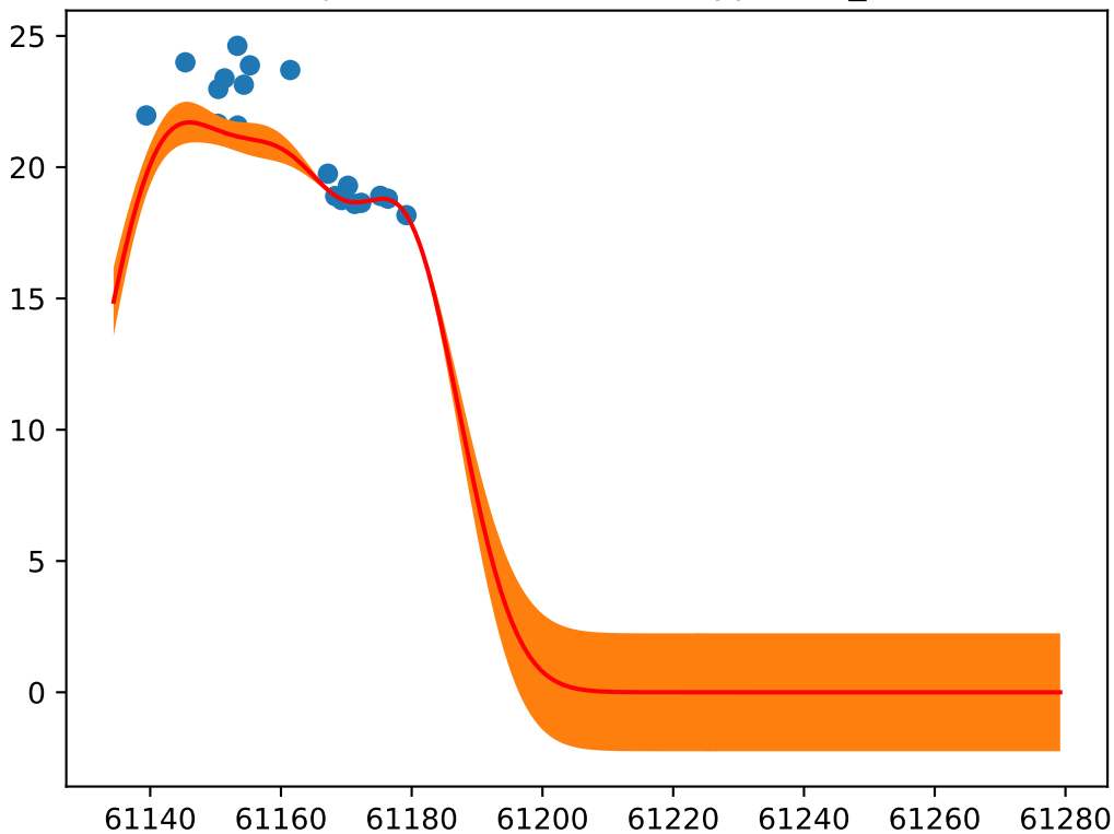
Object: ZTF26aauvdne; Type: SN_Ia
