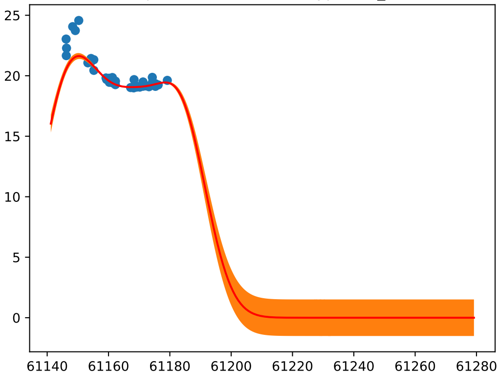
Object: ZTF26aaurnvv; Type: SN_Ia
