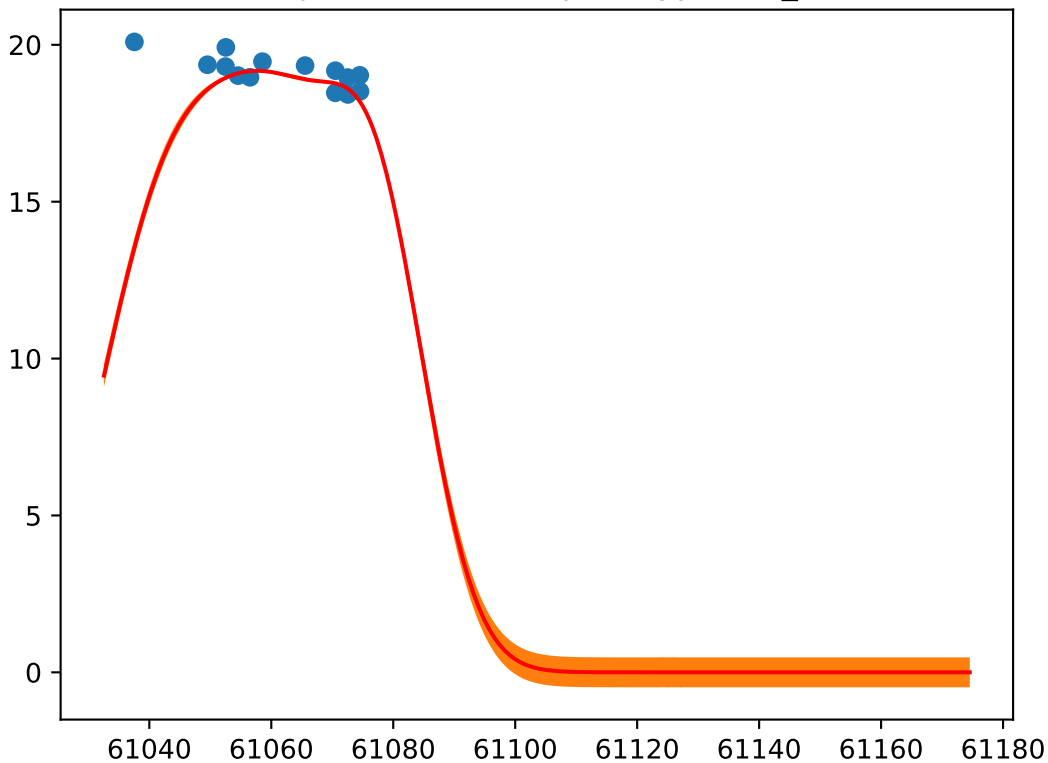
Object: ZTF26aaadpeh; Type: SN_II
