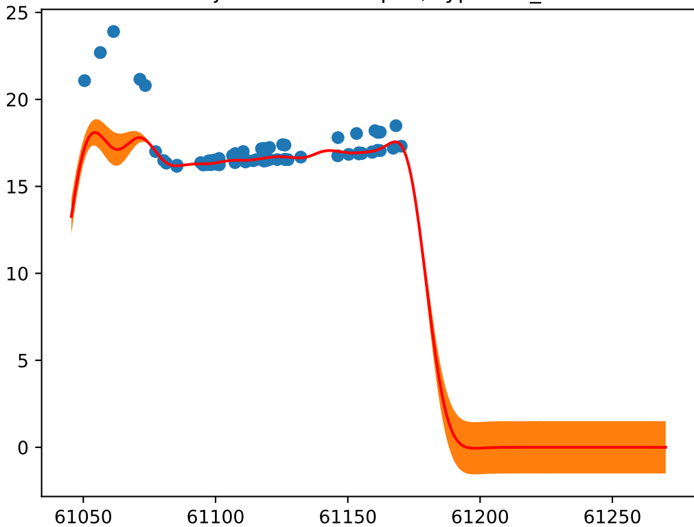
Object: ZTF26aaffpvx; Type: SN_II
