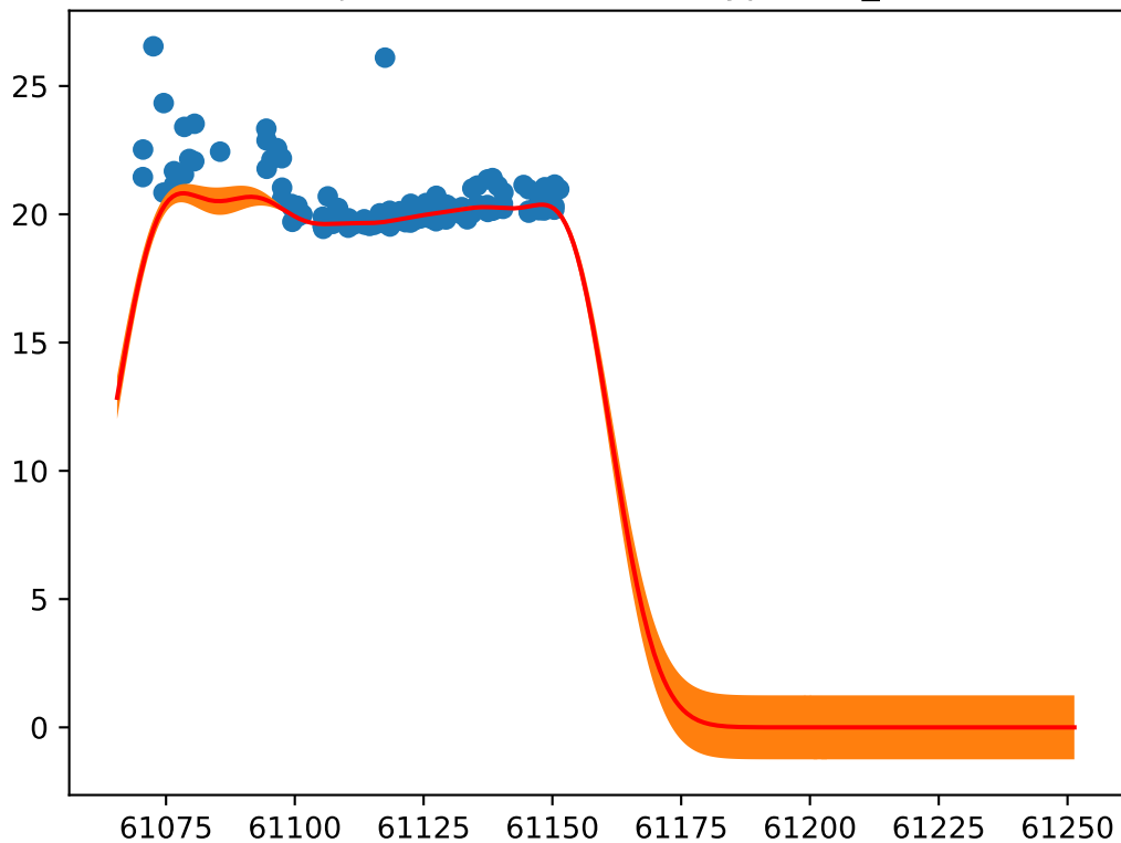
Object: ZTF26aaivdmt; Type: SN_II
