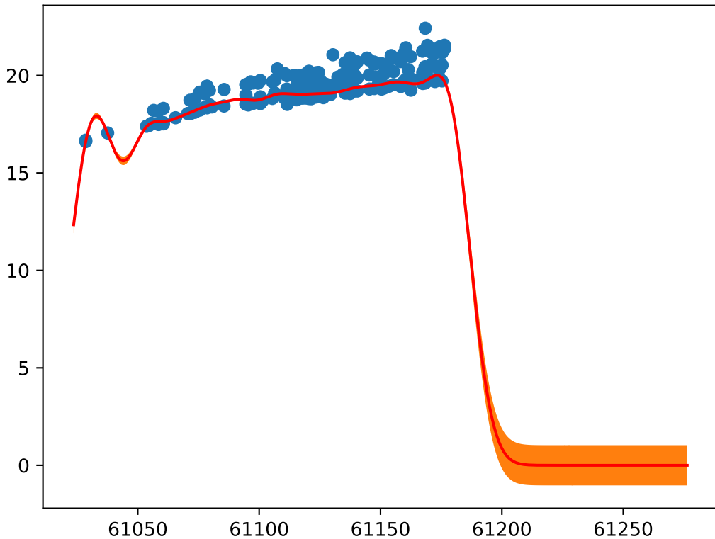
Object: ZTF25acchxhv; Type: SN_II
