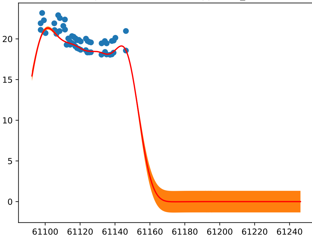
Object: ZTF26aaoanxl; Type: SN_II
