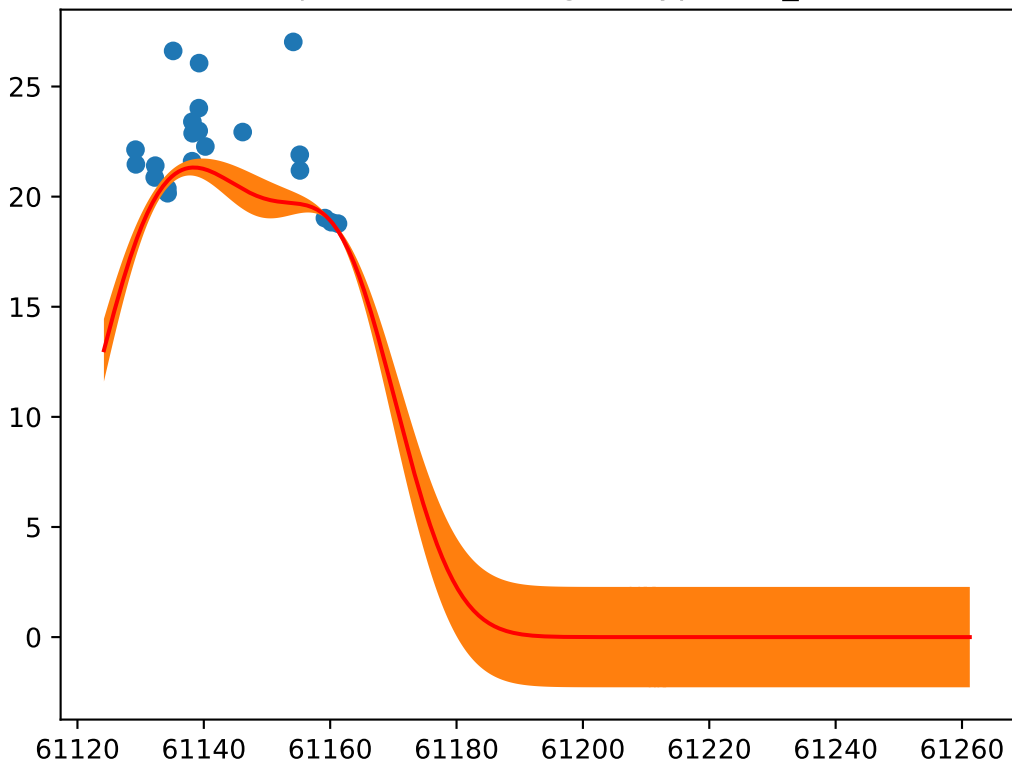
Object: ZTF26aaukgfm; Type: SN_II
