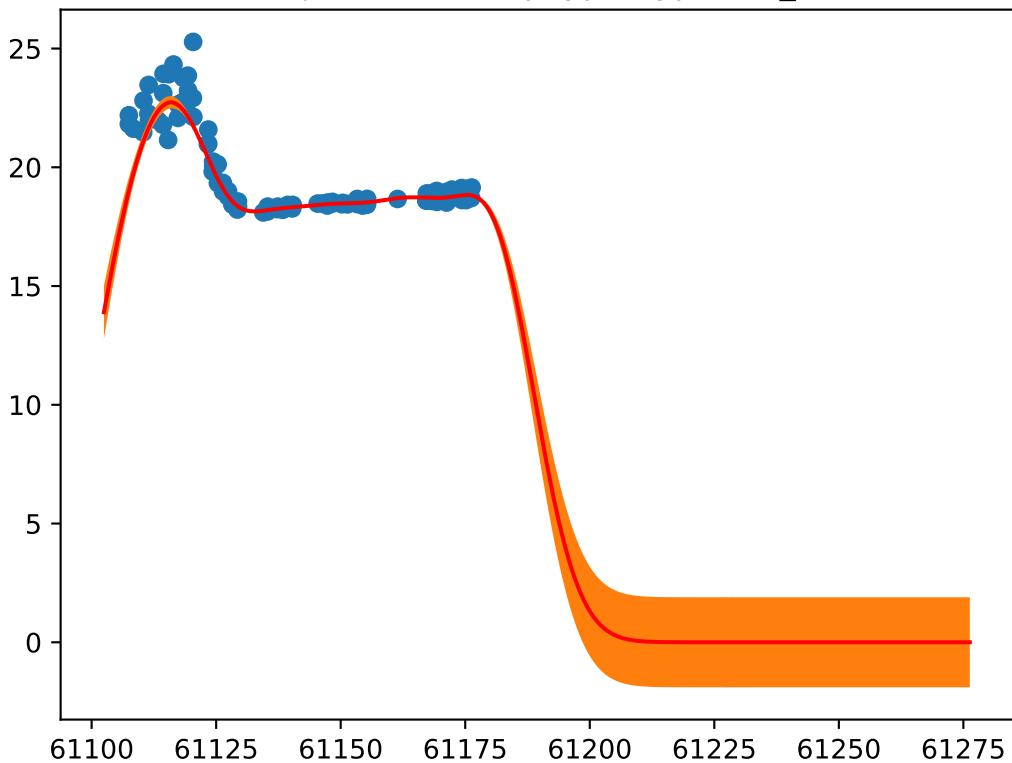
Object: ZTF26aapoypz; Type: SN_II
