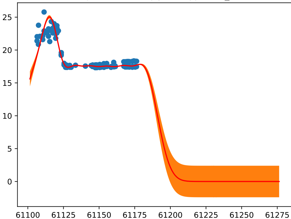
Object: ZTF26aapgvd; Type: SN_II
