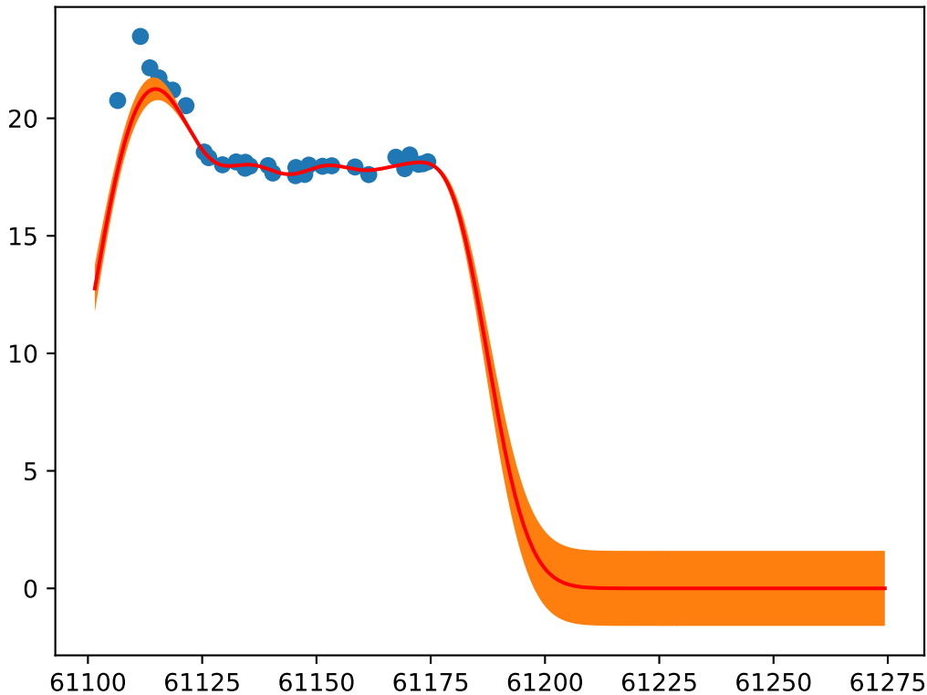
Object: ZTF26aaptccq; Type: SN_II
