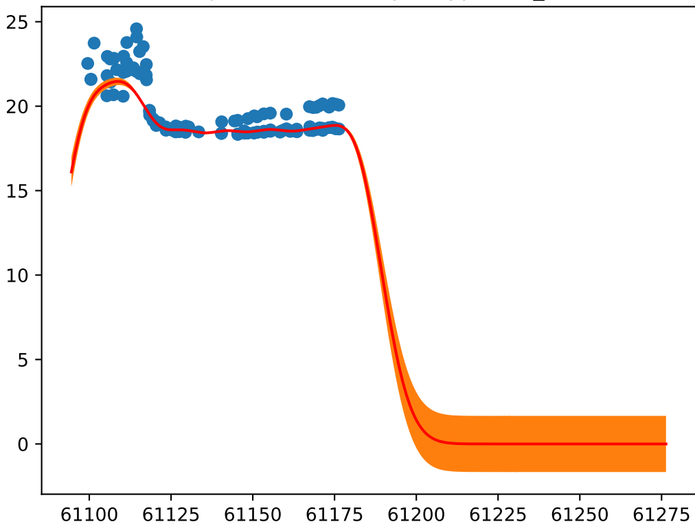
Object: ZTF26aanfqhc; Type: SN_II
