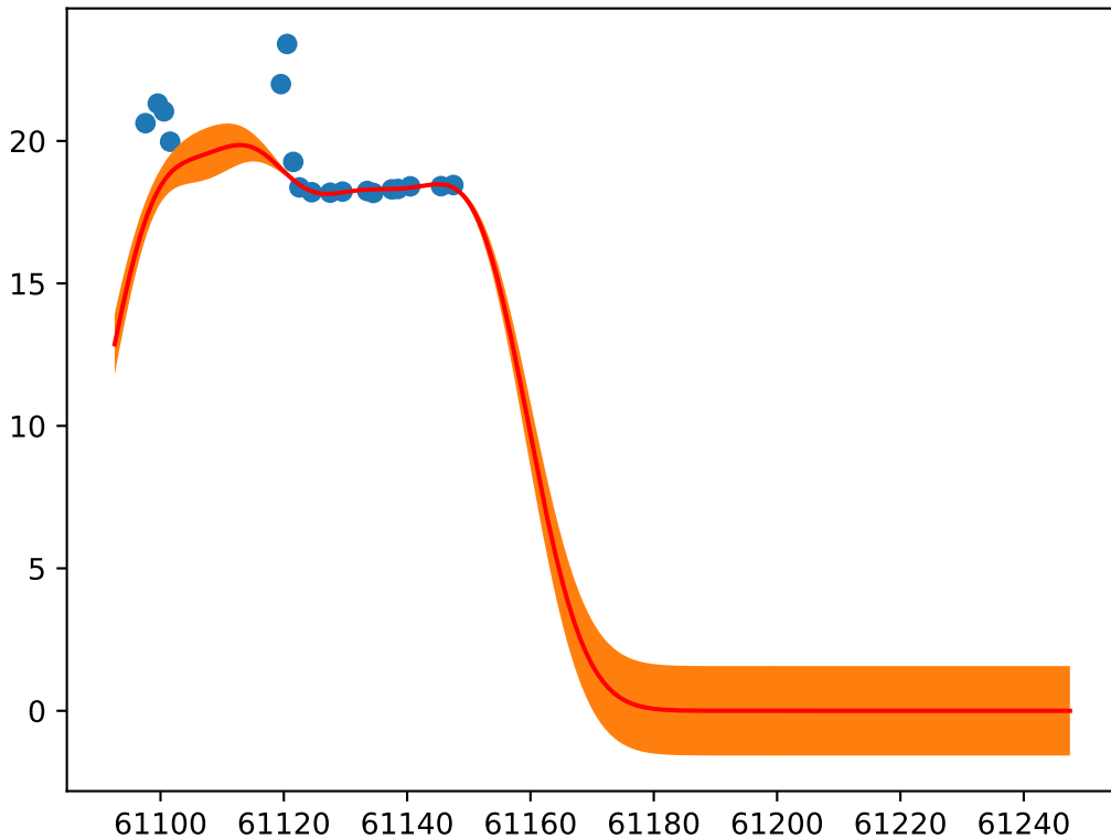
Object: ZTF26aaoqr xr; Type: SN_II
