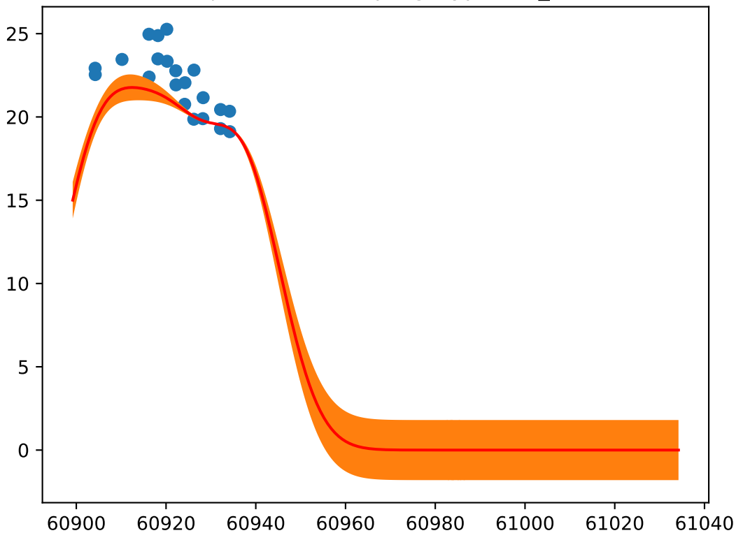
Object: ZTF25abqicvg; Type: SN Ib
