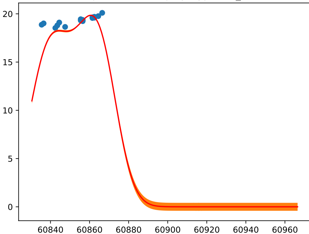
Object: ZTF25aavjchy; Type: SN_Ib
