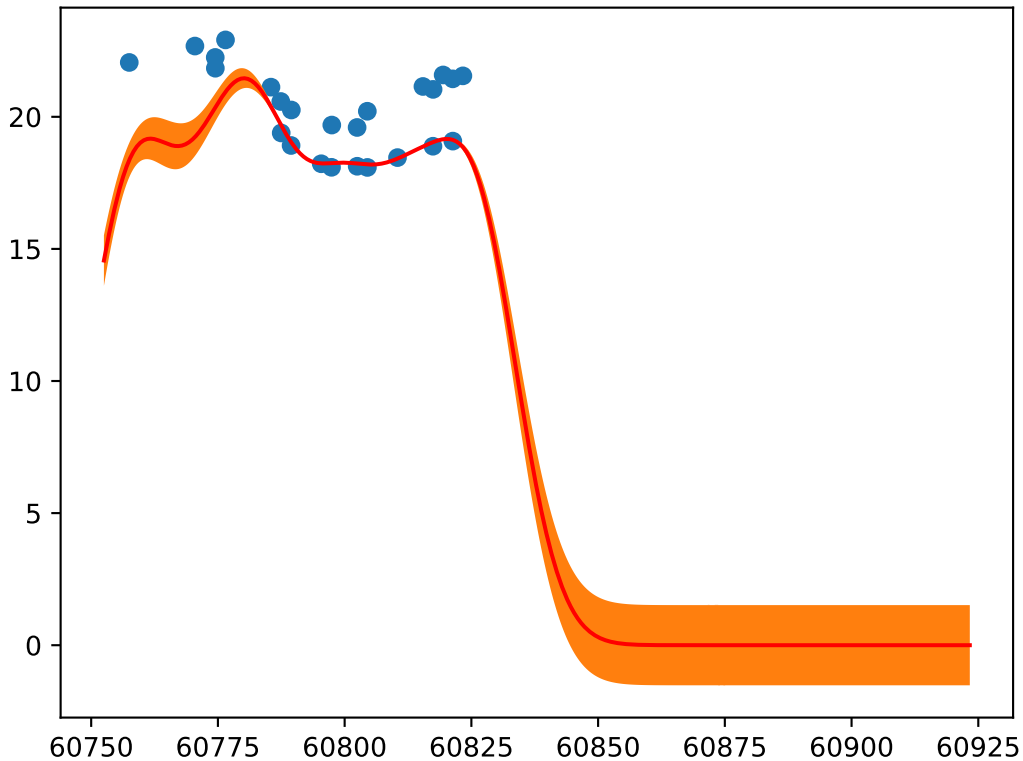
Object: ZTF25aanmfji; Type: SN_Ib
