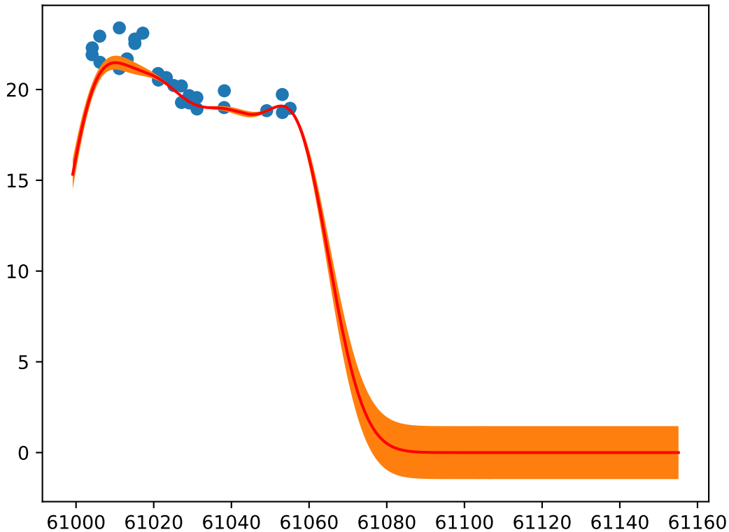
Object: ZTF25acipypu; Type: SN Ib
