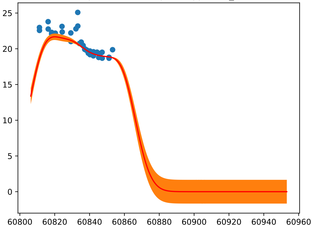
Object: ZTF25aaupzsu; Type: SN_Ic
