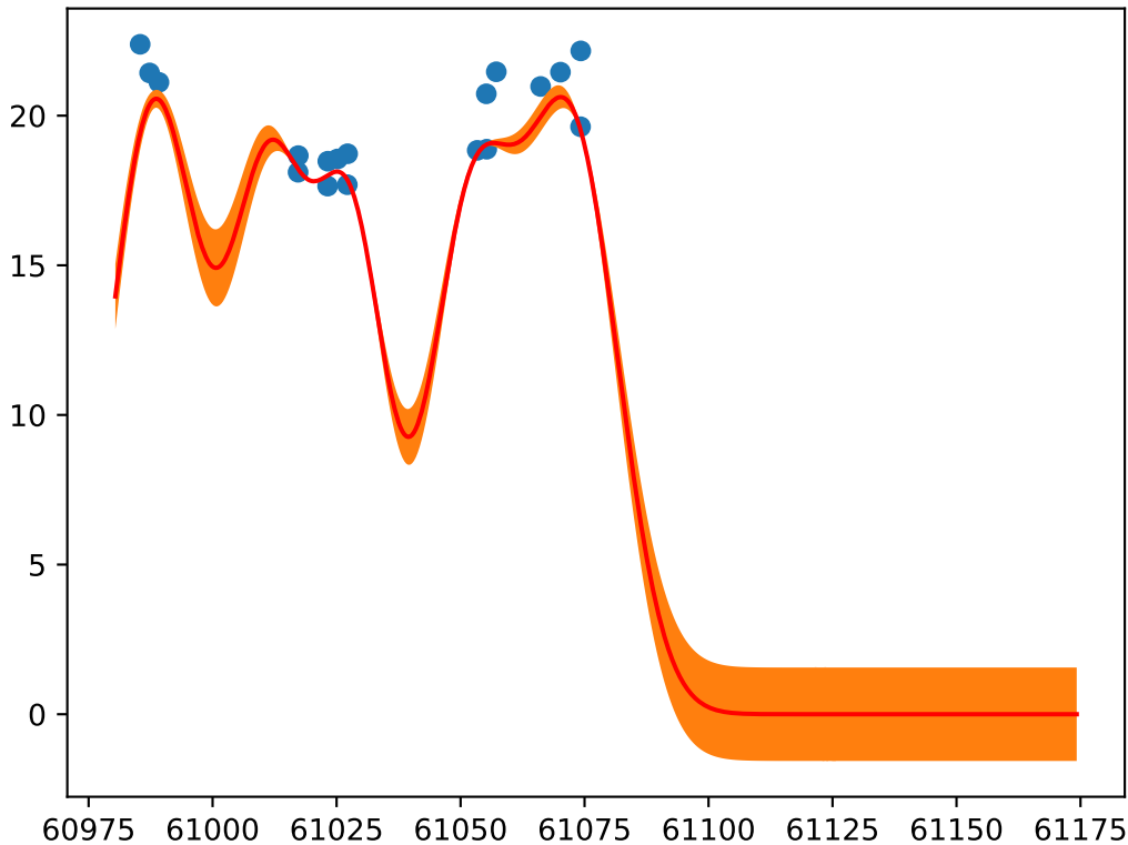
Object: ZTF25acfkoue; Type: SN_Ic
