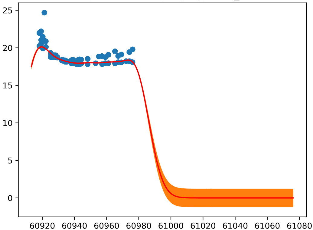
Object: ZTF25abqsbxy; Type: SN_Ic
