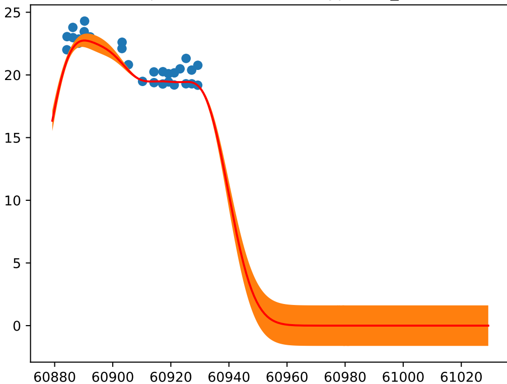
Object: ZTF25abmhftu; Type: SN_Ic
