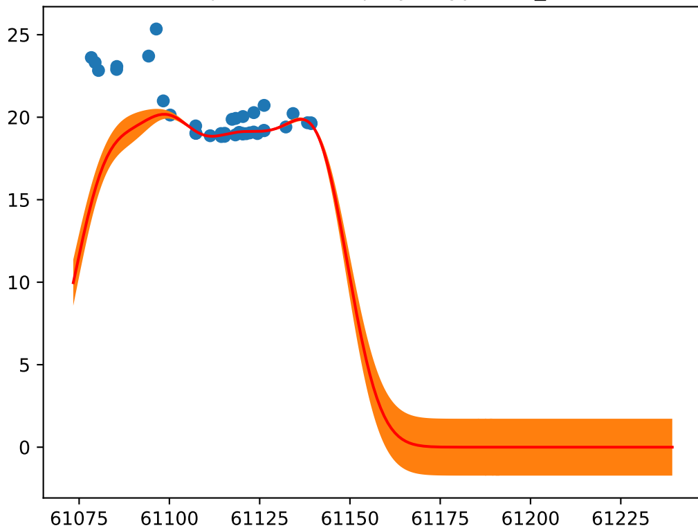
Object: ZTF26aajnayv; Type: SN_Ic
