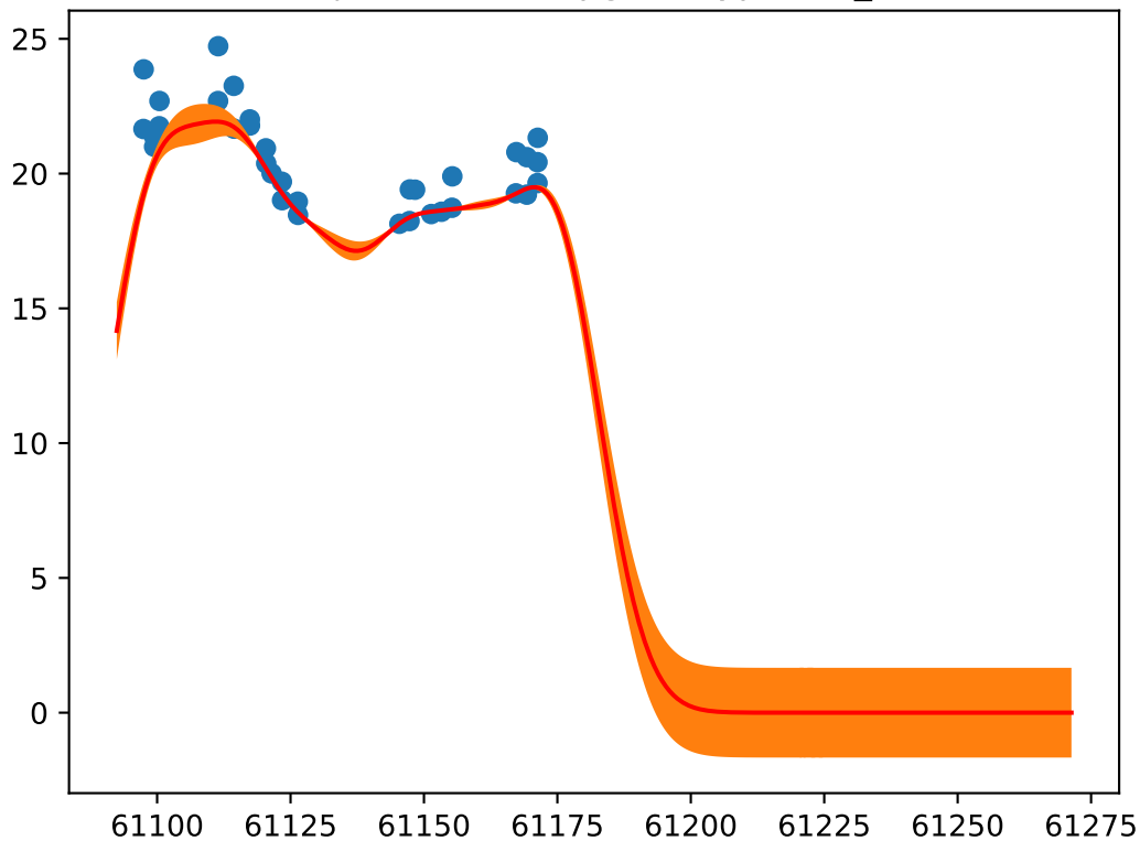
Object: ZTF26aapgavf; Type: SN_Ic
