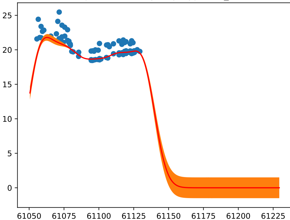
Object: ZTF26aagrmky; Type: SN_Ic
