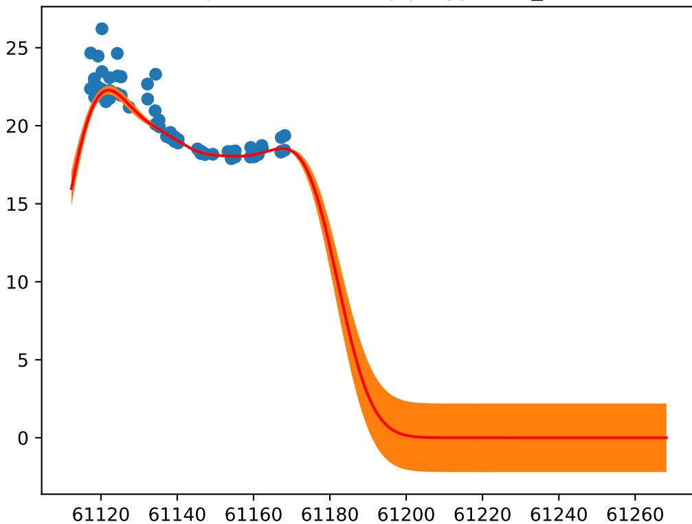
Object: ZTF26aarkqap; Type: SN_Ic
