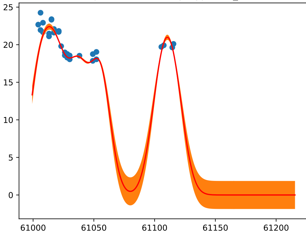
Object: ZTF25achlrsy; Type: SN_Ic
