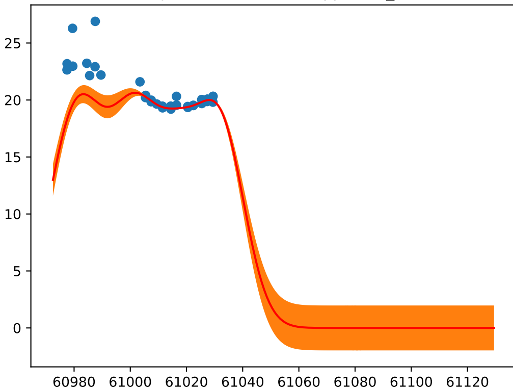
Object: ZTF25acffrxl; Type: SN_Ic
