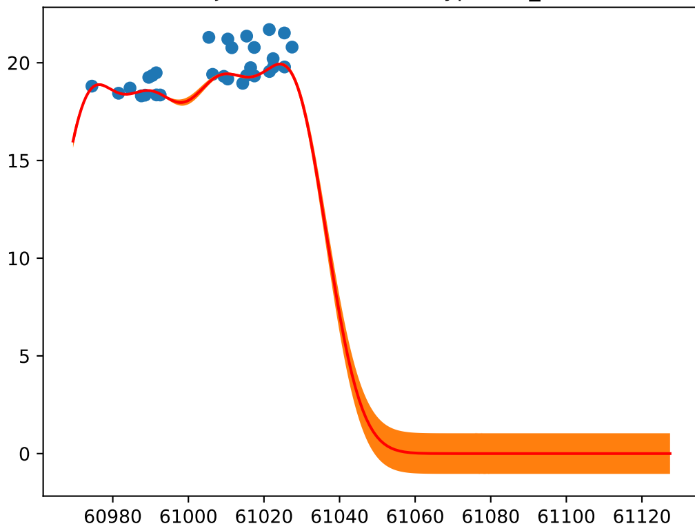
Object: ZTF25abzudli; Type: SN_Ic
