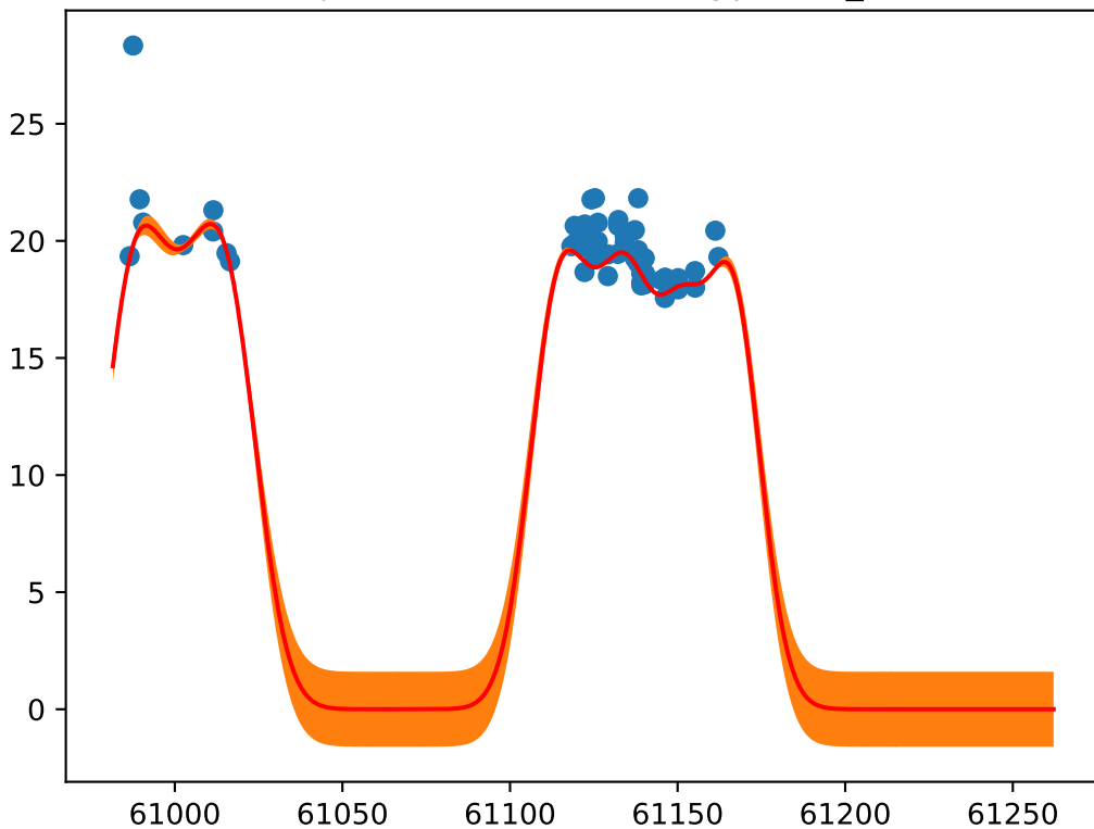
Object: ZTF20acwclnm; Type: SN_Ic
