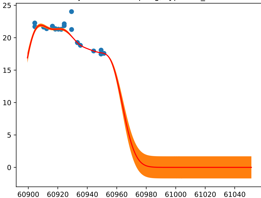
Object: ZTF25abqvssg; Type: SN_Ic
