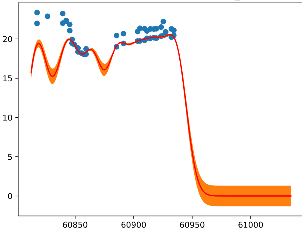
Object: ZTF25aawmdtp; Type: SN_Ic
