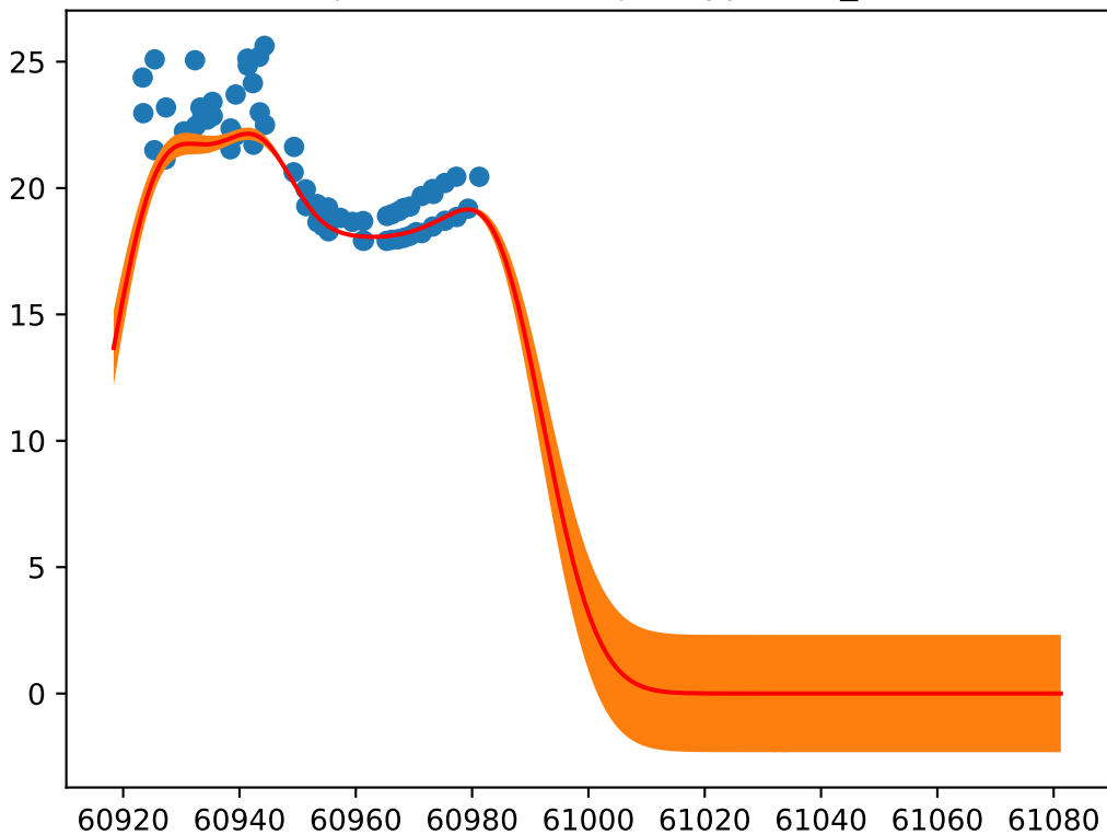
Object: ZTF25abvbjre; Type: SN_Ic
