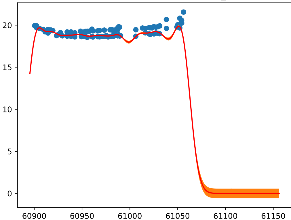
Object: ZTF25abitcpd; Type: SN_Ic
