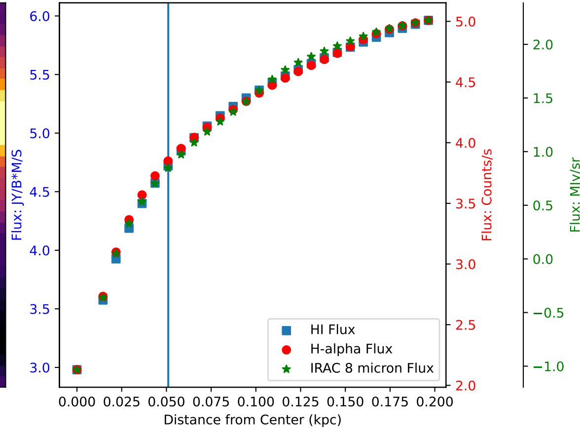
Flux of HI vs. H-alpha in Galaxy: WLM - Region 3
