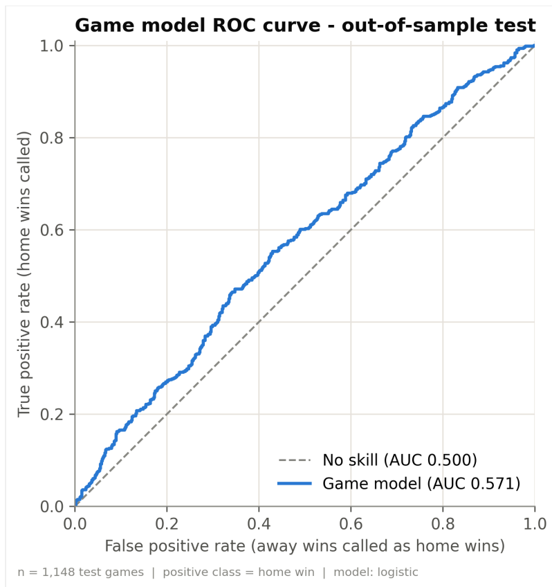
Figure 2. ROC Curve for Game-Level Win Predictions
