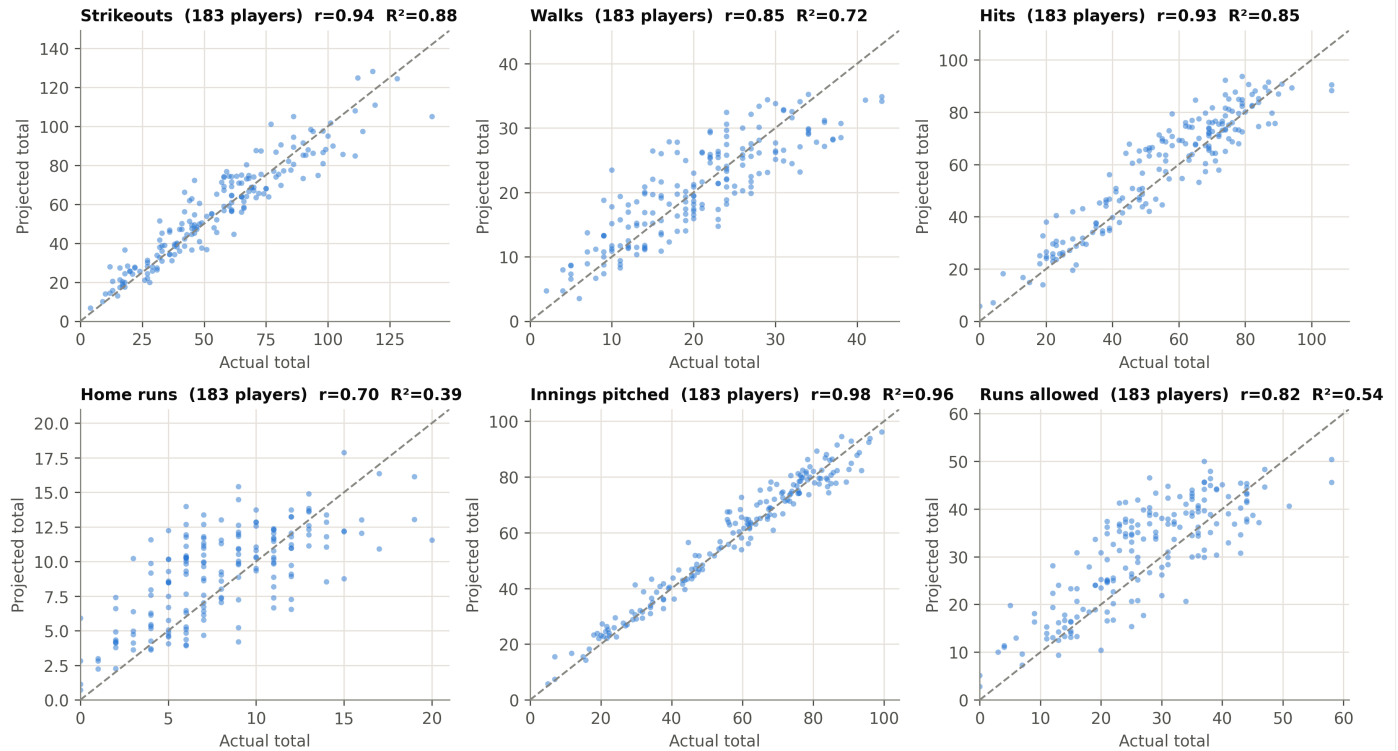
Figure 5. Predicted vs. Actual Pitcher Totals
