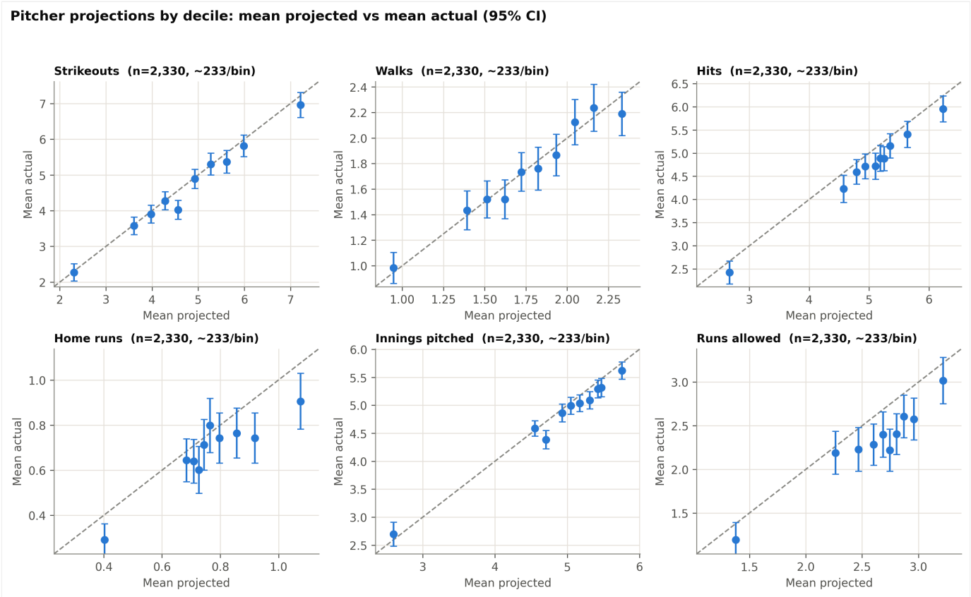
Figure 3. Pitcher Projection Calibration by Decile
