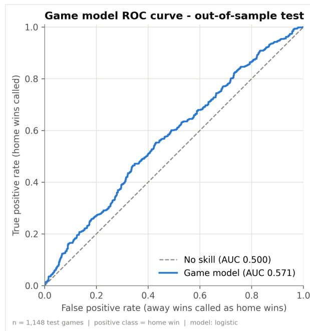
Figure 2. ROC Curve for Game-Level Win Predictions
