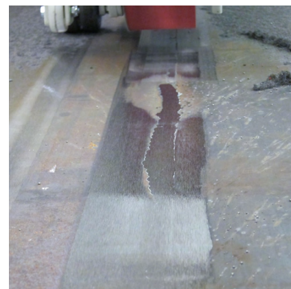
__ after belt grinding of plate with CLF75
