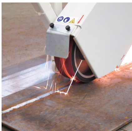
__ contact roller movable machine for grinding heavy plates
