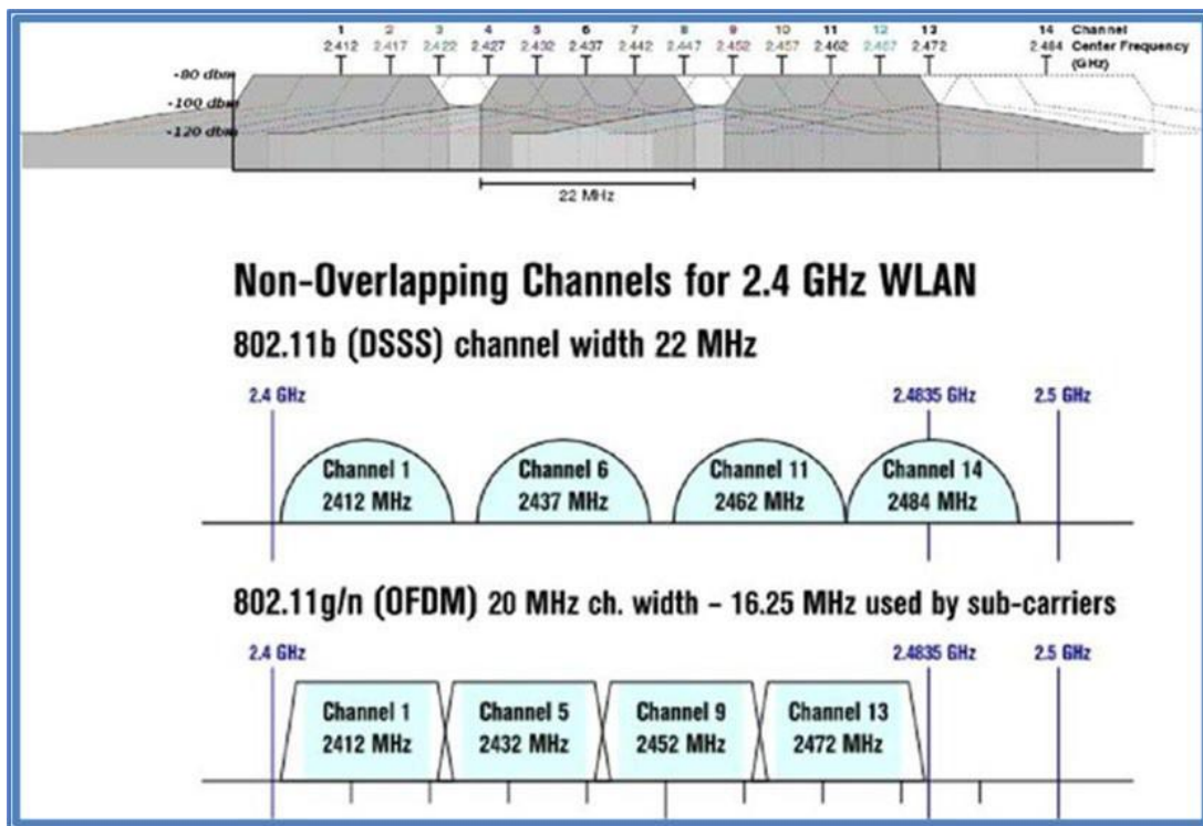
Figure 12 Communication Channels
