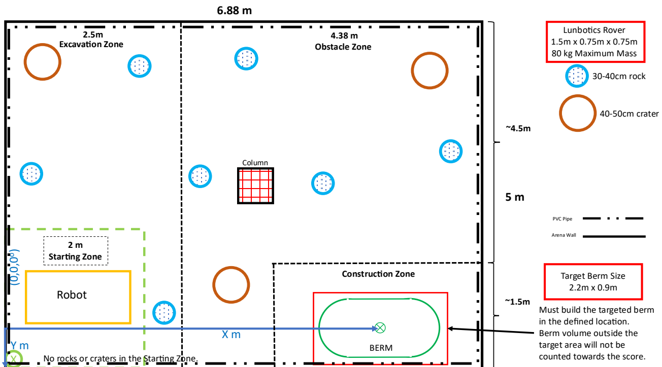
Figure 9 Arena Dimensions and Obstacle Layout
