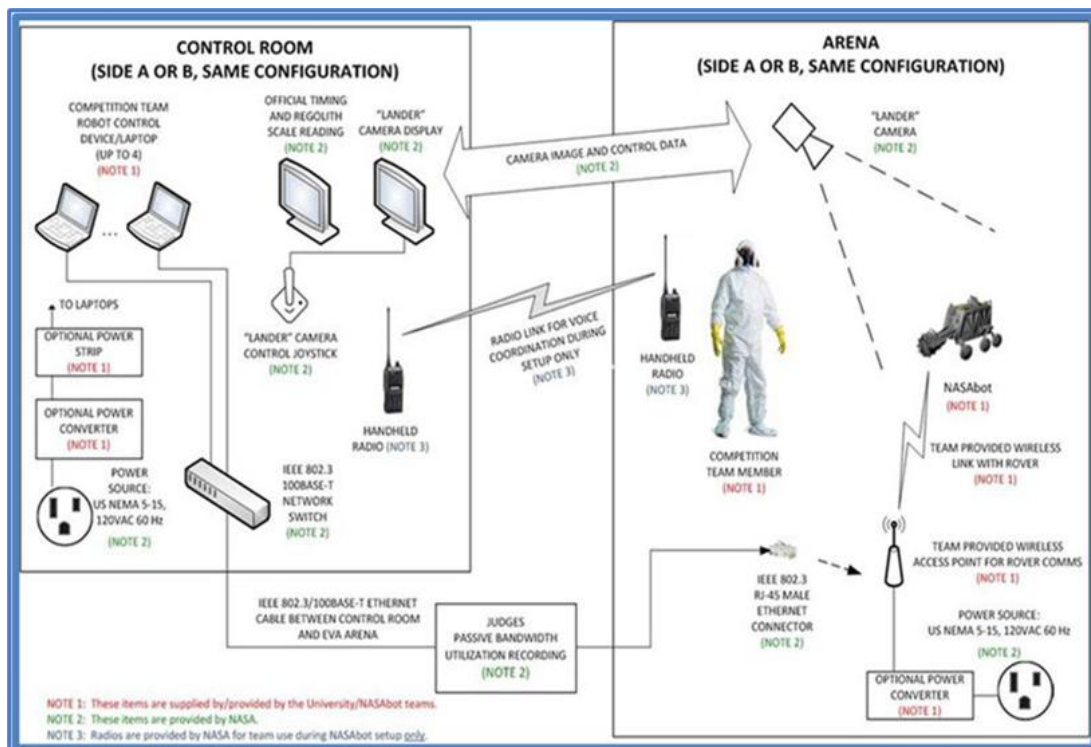
Figure 13 Comm Configuration
