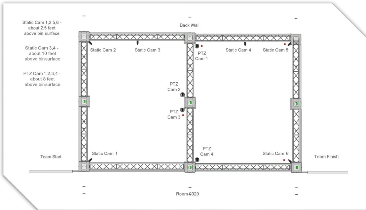
Figure 10 Arena Camera Layout
