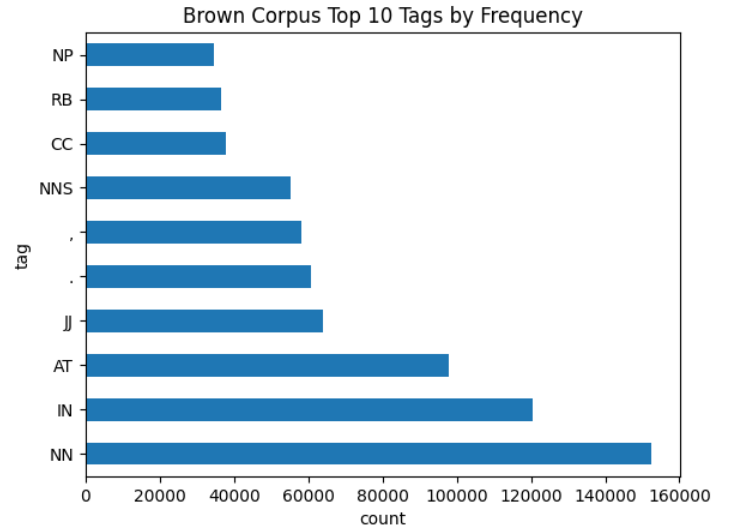
Figure 1: Top ten POS tags by frequency
