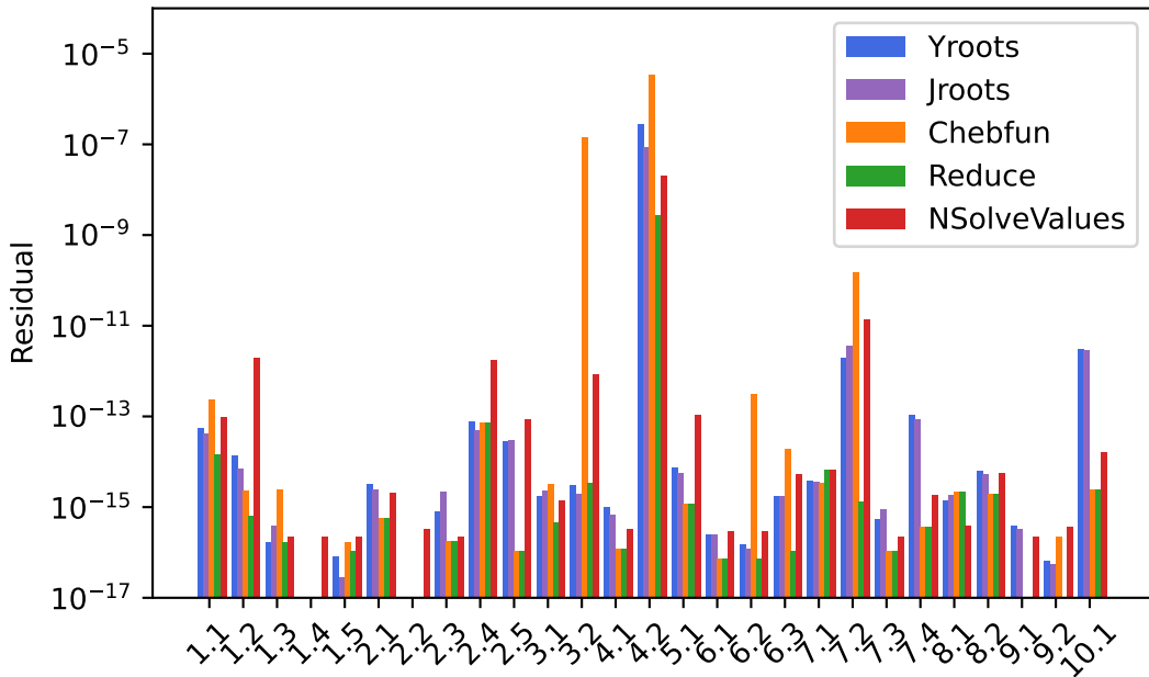
Chebfun Suite Maximum Residuals
