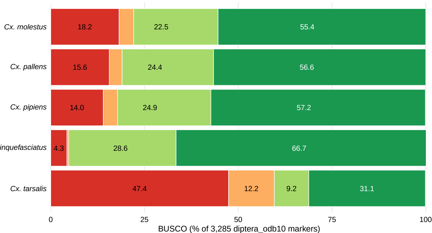
(a) Protein-mode BUSCO completeness
