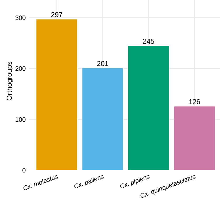
(c) Form-specific cloud orthogroups
