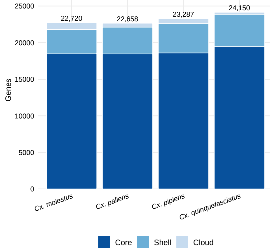
(b) Genes per species by compartment
