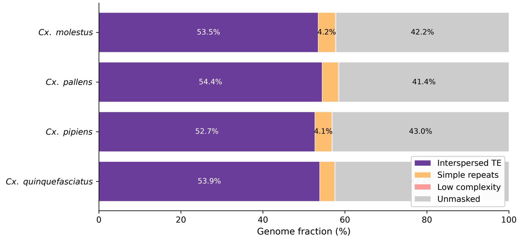
Figure 6. Repeat composition across Culex pipiens complex genomes
