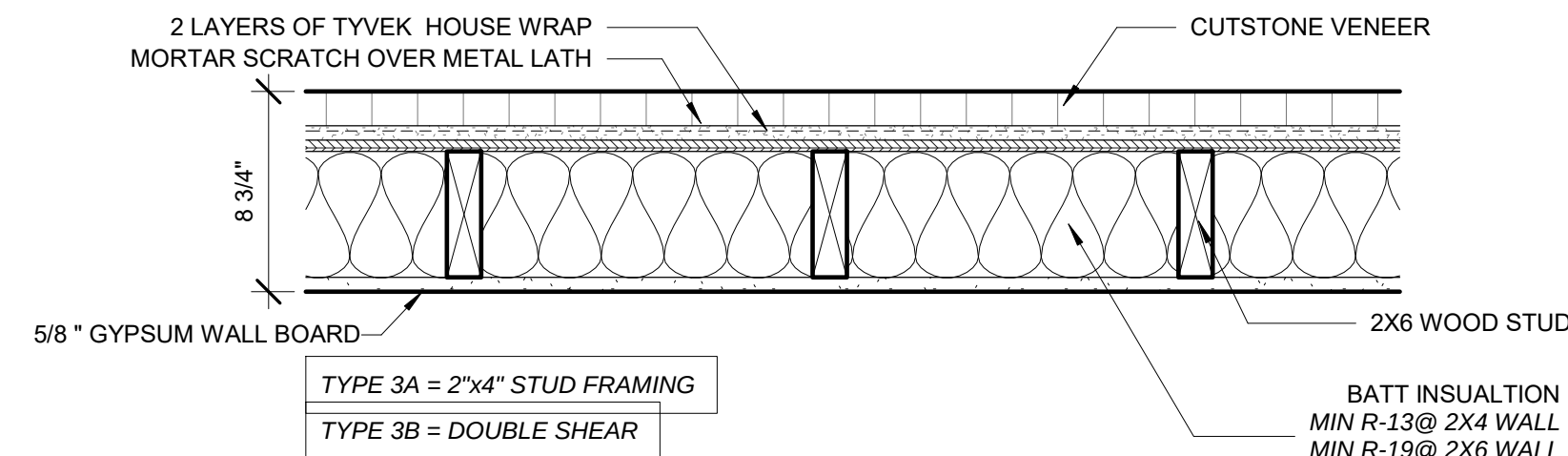
3 EXTERIOR SHEAR STONE VENEER 1 1/2" = 1'-0"
