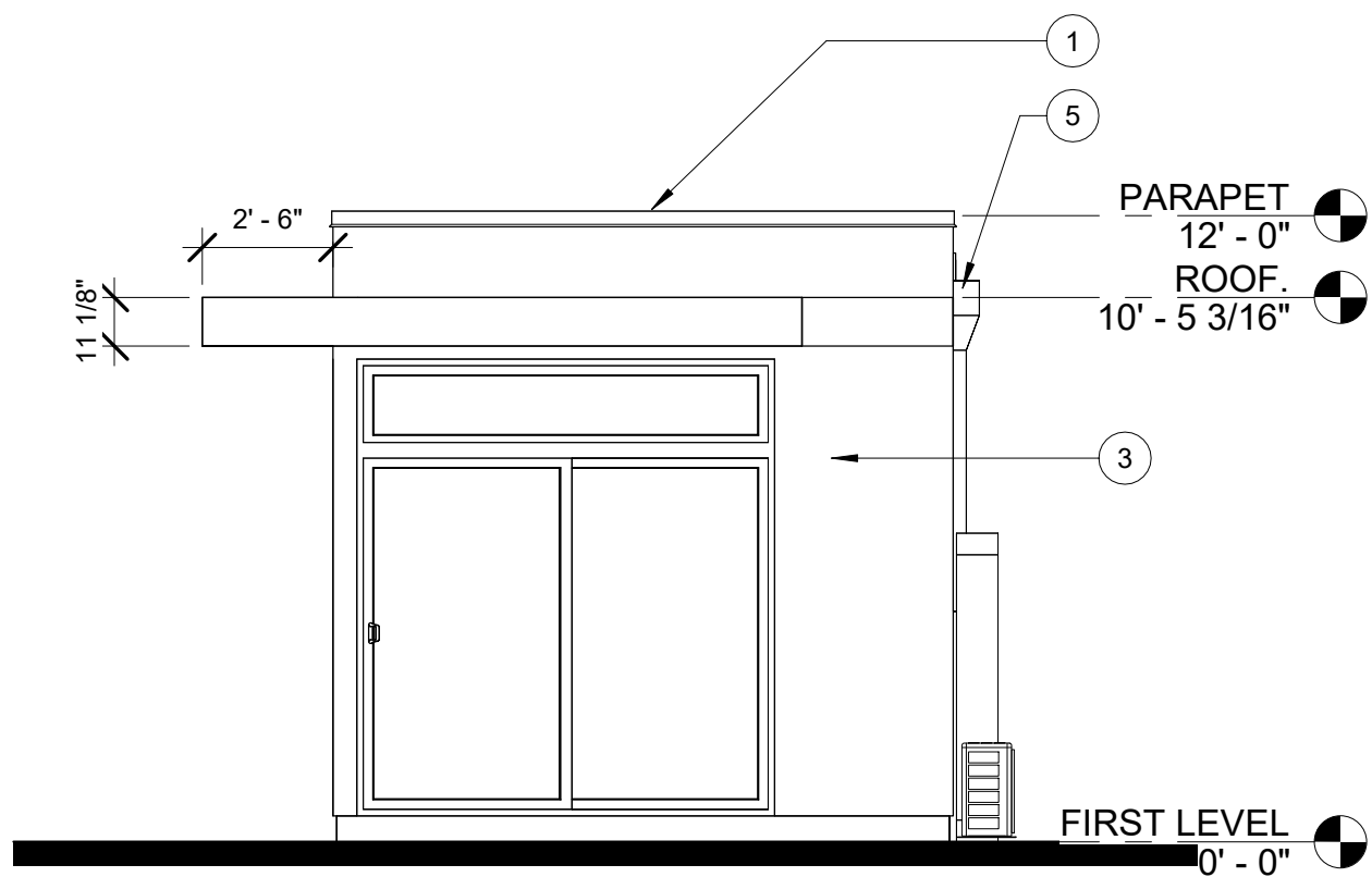
③ DETACHED BLDG SOUTH ELEVATION 1/4" = 1'-0"
