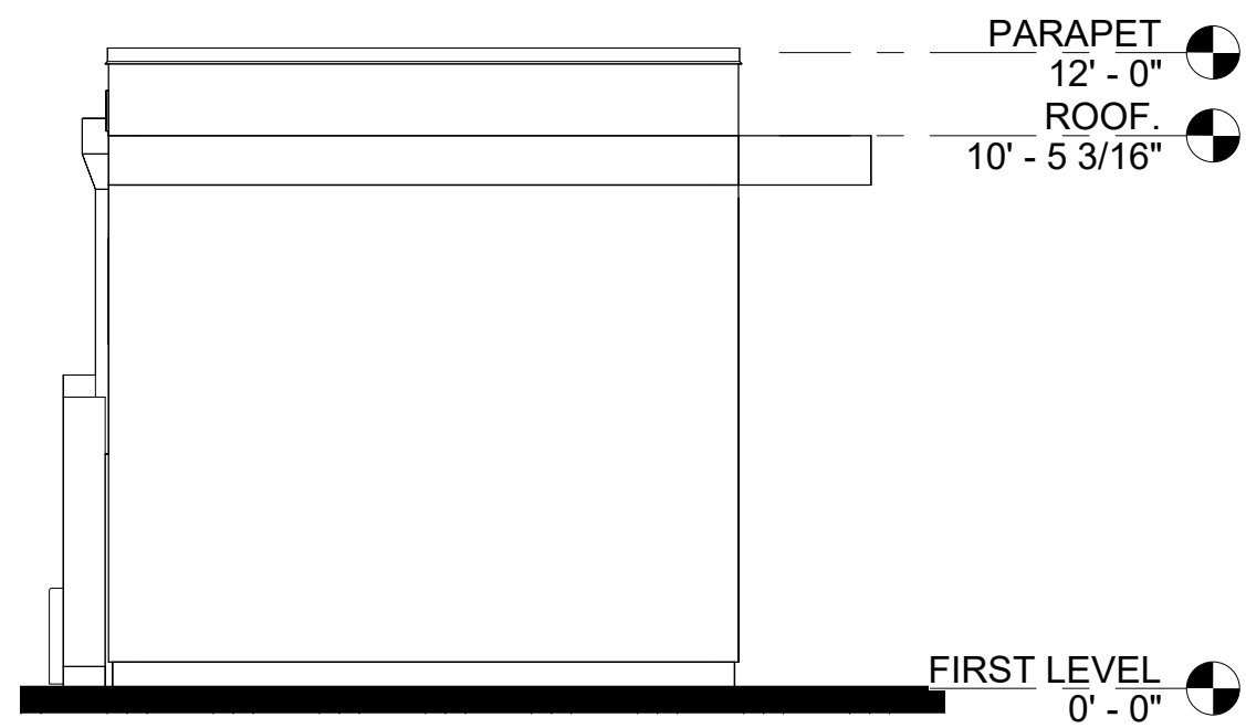
④ DETACHED BLDG NORTH ELEVATION 1/4" = 1'-0"
