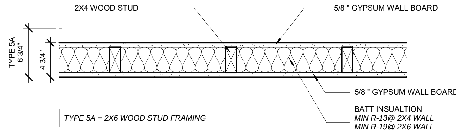
5 INTERIOR WALL 1 1/2" = 1'-0"
