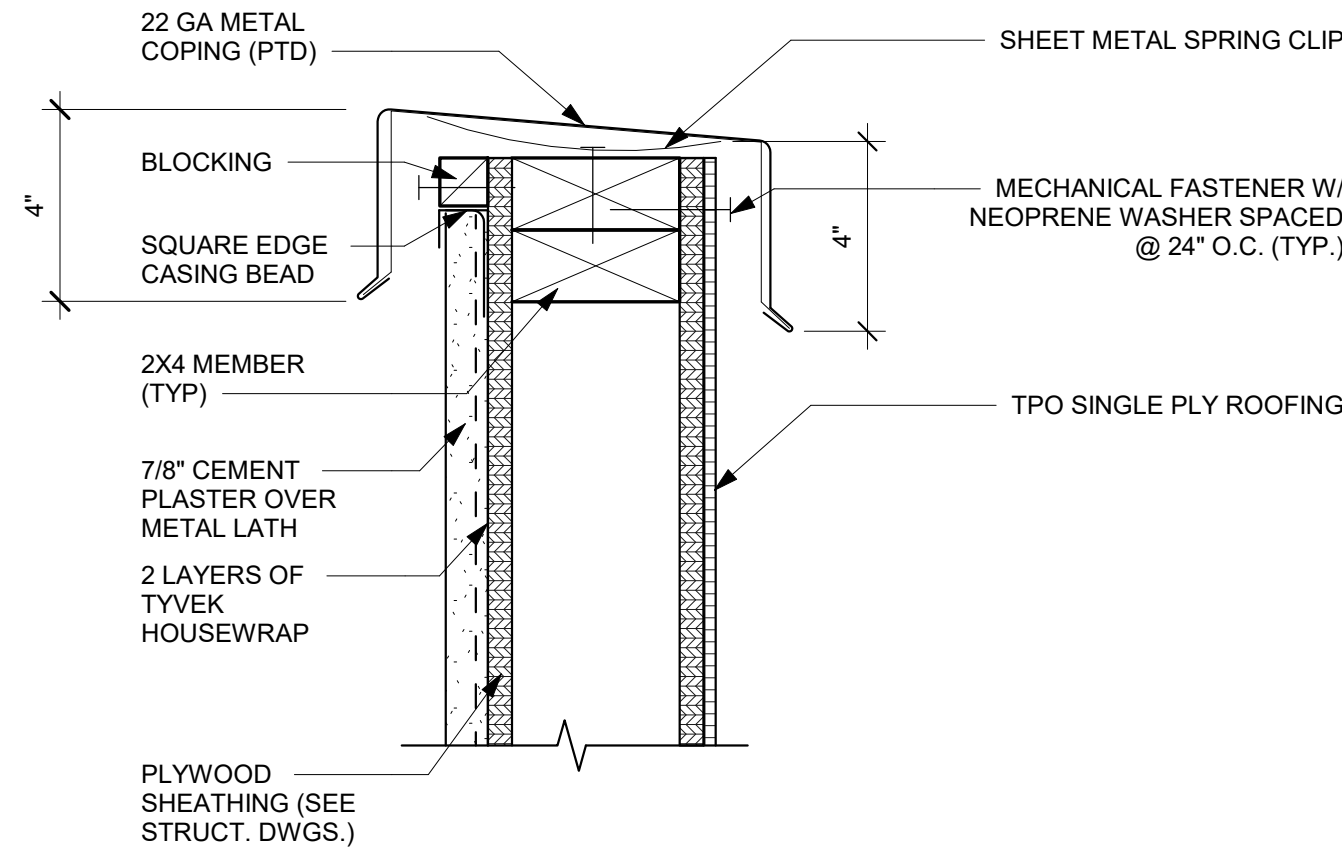
3 PARAPET COPING DETAIL 3" = 1'-0"
