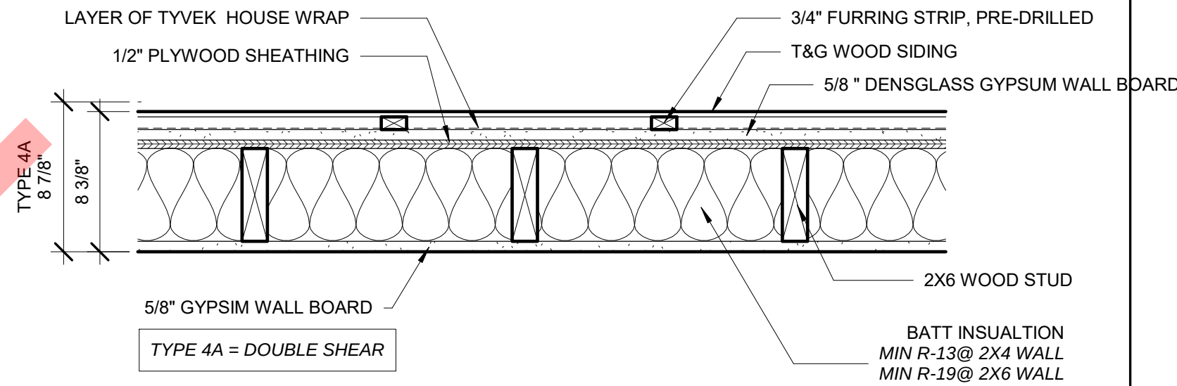
4 EXTERIOR SHEAR W/WOOD SIDING 1 1/2" = 1'-0"
