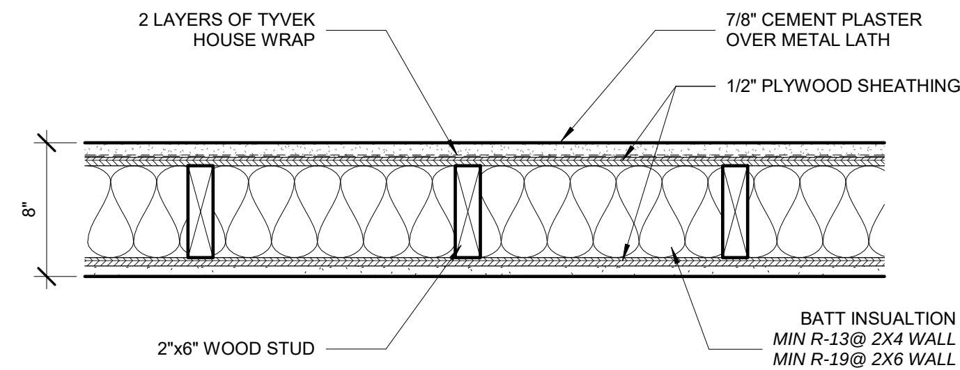
2 EXTERIOR DOUBLE SHEAR (1-HR) 1 1/2" = 1'-0"
