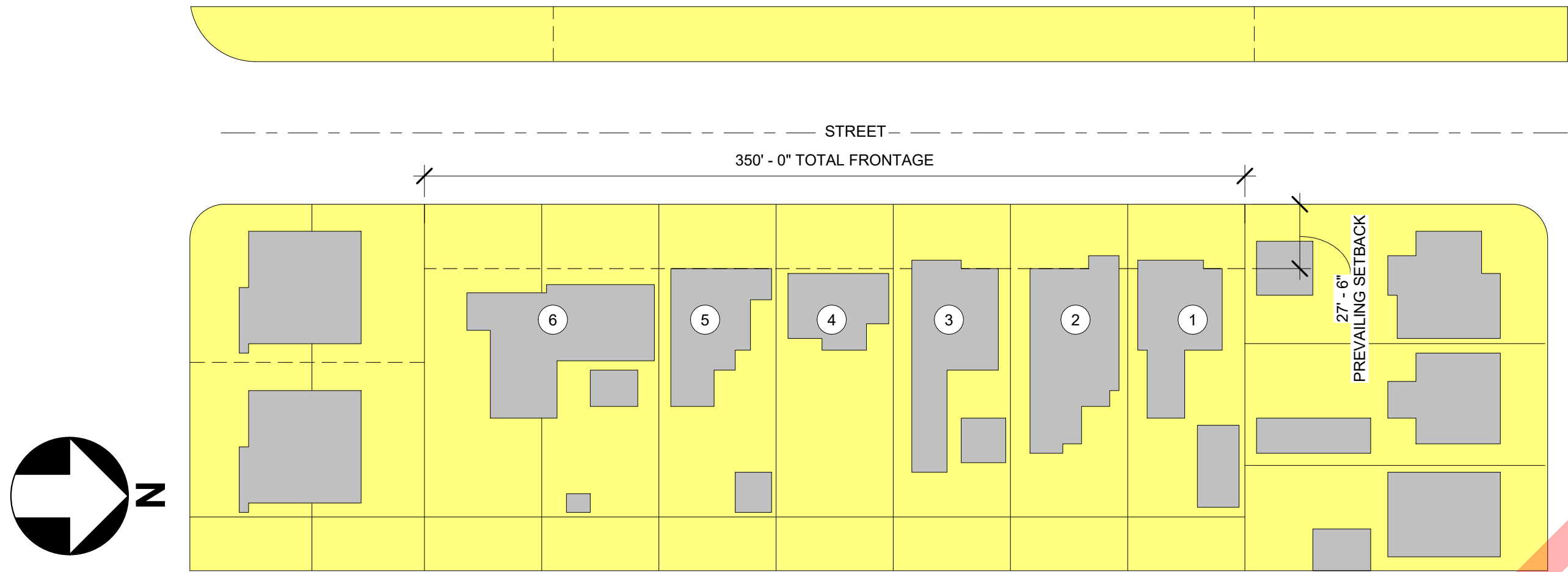
3 FRONTAGE 1" = 50'-0"
