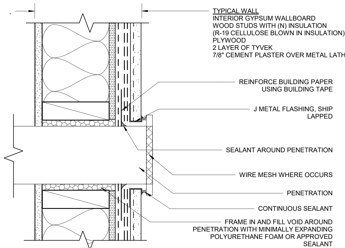
2 WALL PENETRATION DETAIL 3" = 1'-0"
