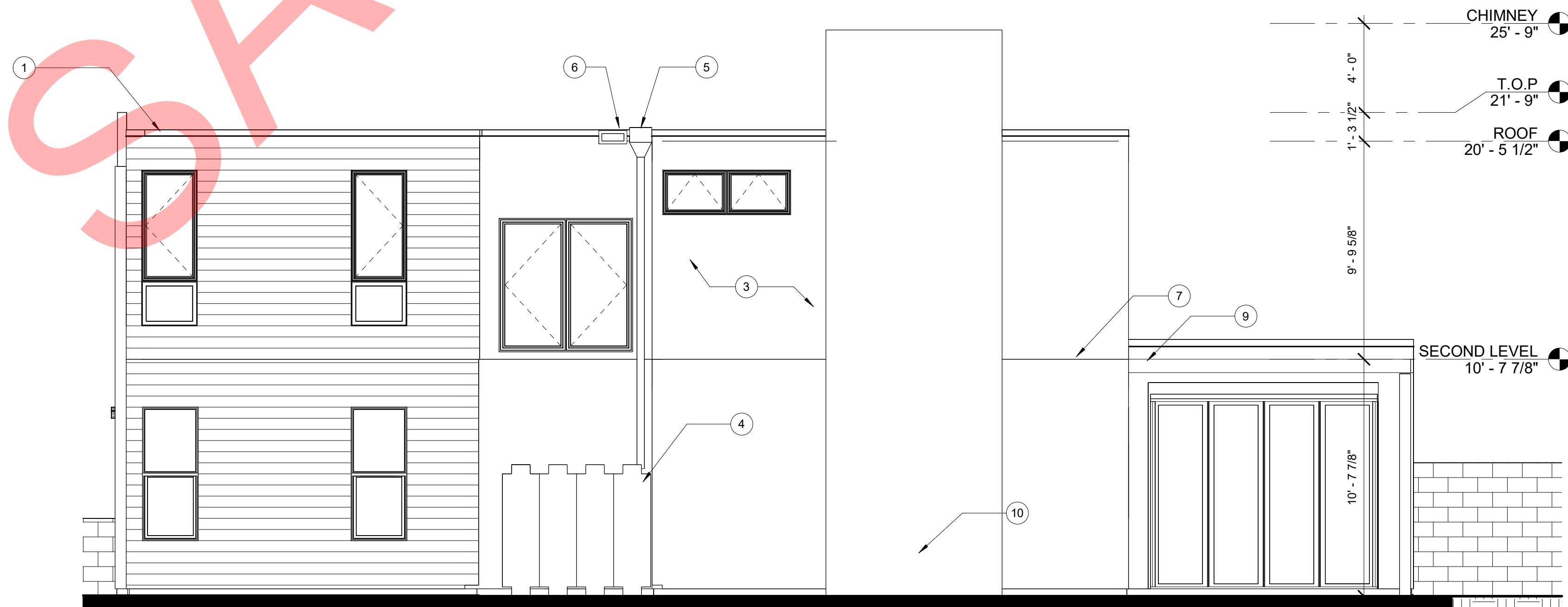
① SOUTH ELEVATION 1/4" = 1'-0"
