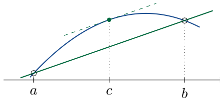
Figure 8.4.8. MEAN VALUE THEOREM. Some interior tangent is parallel to the chord joining the endpoints.
